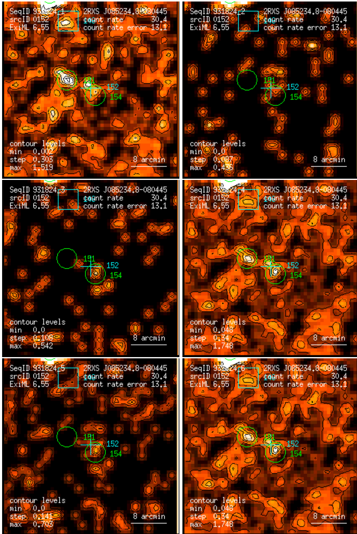
Figure 152: RASS 931824: detection 0152: band rate images, Gaussian filter: (1) PSPC channels 11 – 41, (2) 52 – 90, (3) 91 – 201, (4) 11 – 235, (5) 52 – 201, (6) 11 – 201. Broad band rates in counts/ks. Band rate contour levels in counts/ks/arcmin 2 .
