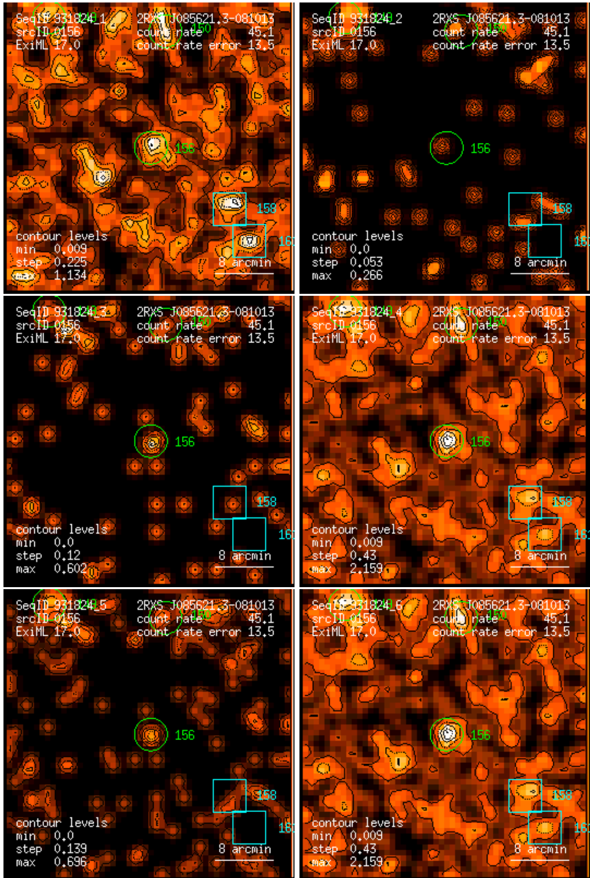
Figure 156: RASS 931824: detection 0156: band rate images, Gaussian filter: (1) PSPC channels 11 – 41, (2) 52 – 90, (3) 91 – 201, (4) 11 – 235, (5) 52 – 201, (6) 11 – 201. Broad band rates in counts/ks. Band rate contour levels in counts/ks/arcmin 2 .
