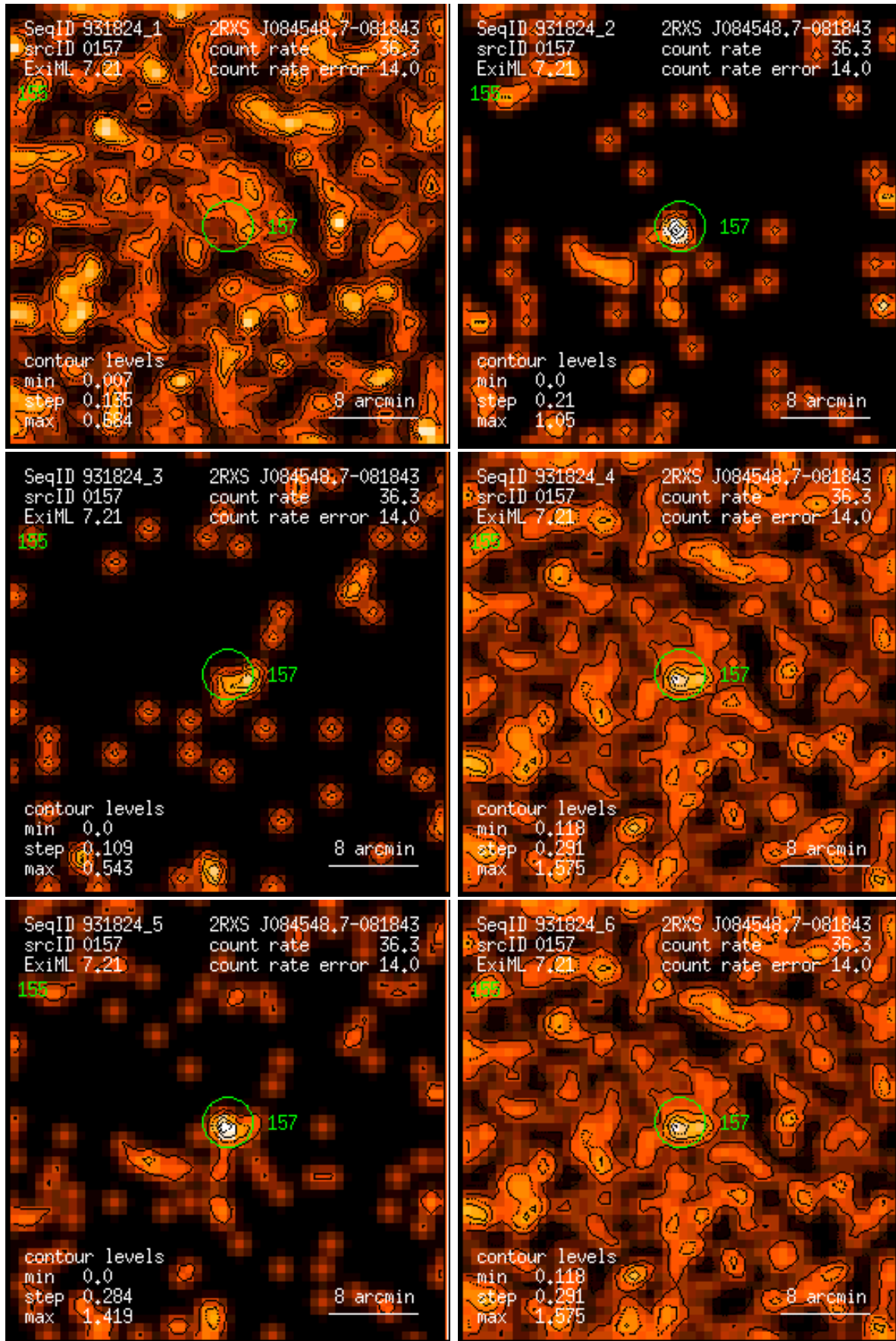
Figure 157: RASS 931824: detection 0157: band rate images, Gaussian filter: (1) PSPC channels 11 – 41, (2) 52 – 90, (3) 91 – 201, (4) 11 – 235, (5) 52 – 201, (6) 11 – 201. Broad band rates in counts/ks. Band rate contour levels in counts/ks/arcmin 2 .
