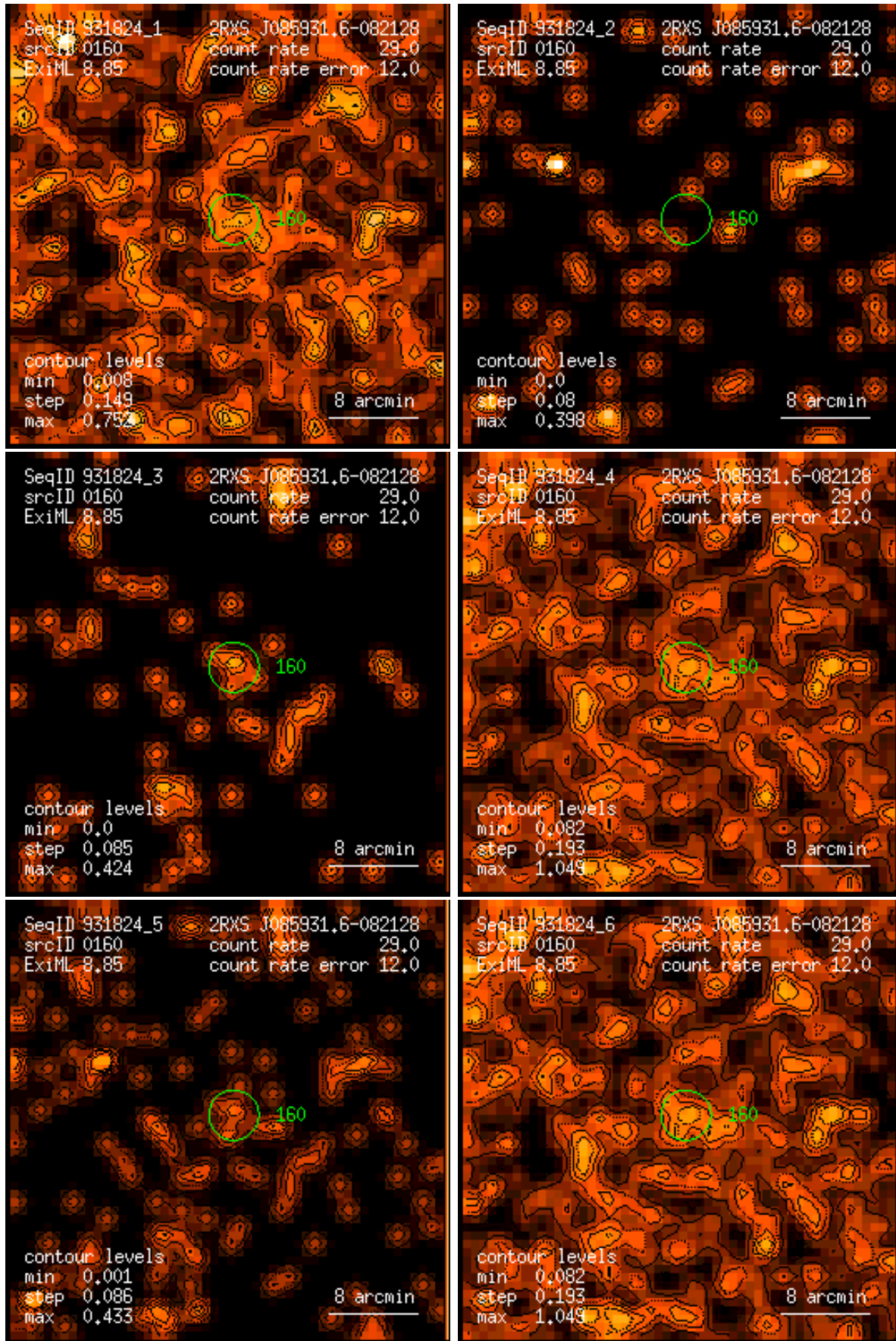
Figure 160: RASS 931824: detection 0160: band rate images, Gaussian filter: (1) PSPC channels 11 – 41, (2) 52 – 90, (3) 91 – 201, (4) 11 – 235, (5) 52 – 201, (6) 11 – 201. Broad band rates in counts/ks. Band rate contour levels in counts/ks/arcmin 2 .
