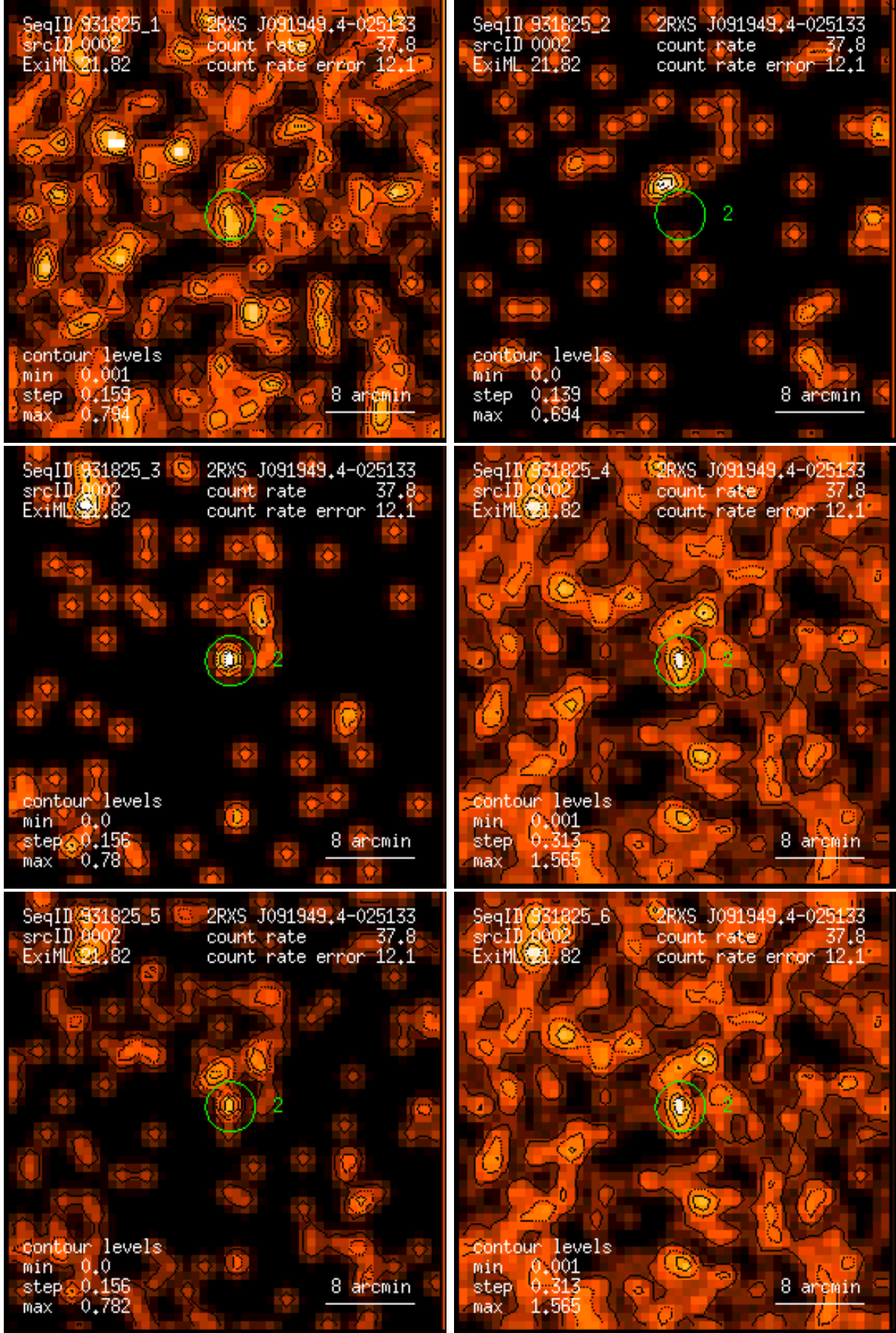
Figure 2: RASS 931825: detection 0002: band rate images, Gaussian filter: (1) PSPC channels 11 – 41, (2) 52 – 90, (3) 91 – 201, (4) 11 – 235, (5) 52 – 201, (6) 11 – 201. Broad band rates in counts/ks. Band rate contour levels in counts/ks/arcmin 2 .
