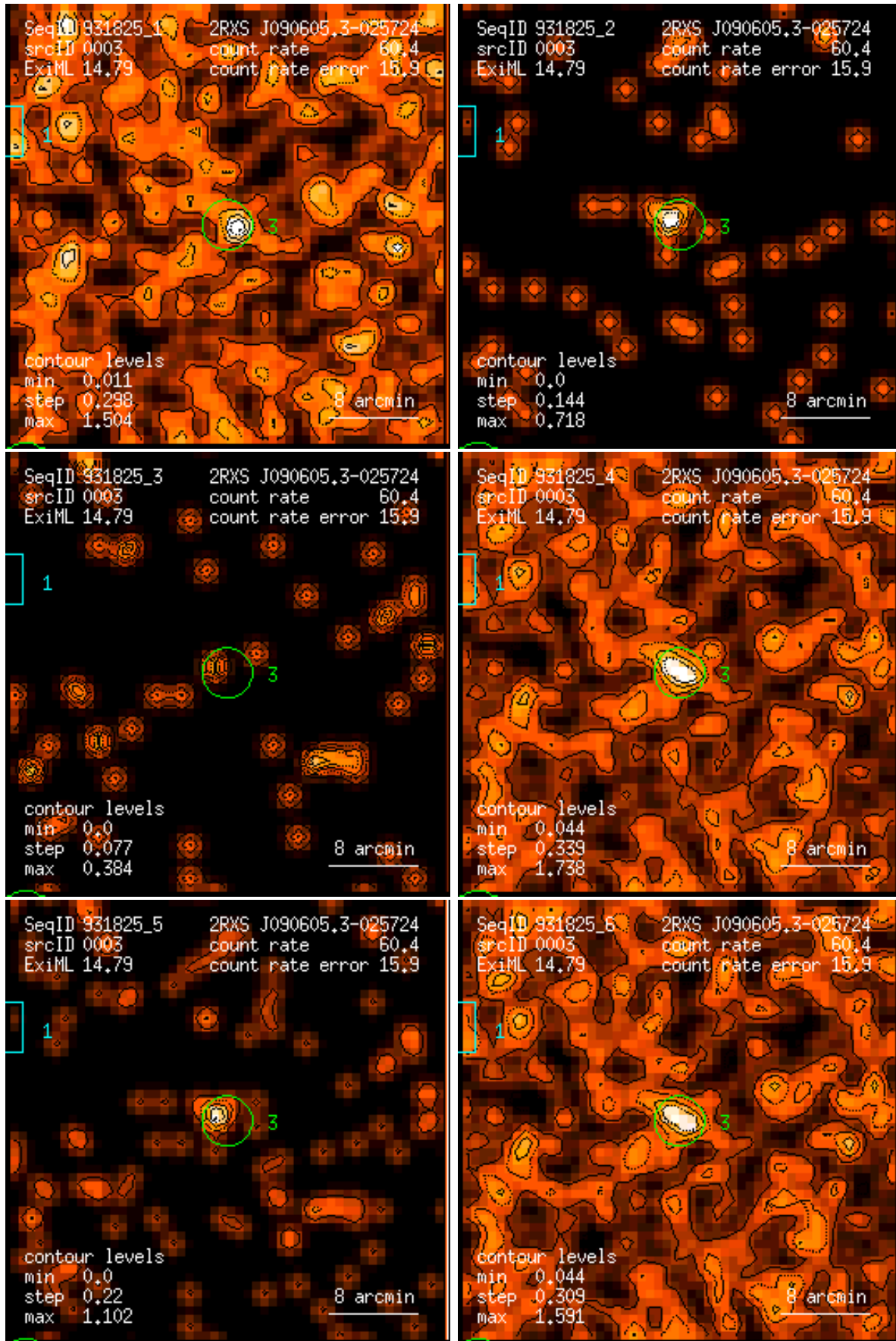
Figure 3: RASS 931825: detection 0003: band rate images, Gaussian filter: (1) PSPC channels 11 – 41, (2) 52 – 90, (3) 91 – 201, (4) 11 – 235, (5) 52 – 201, (6) 11 – 201. Broad band rates in counts/ks. Band rate contour levels in counts/ks/arcmin 2 .
