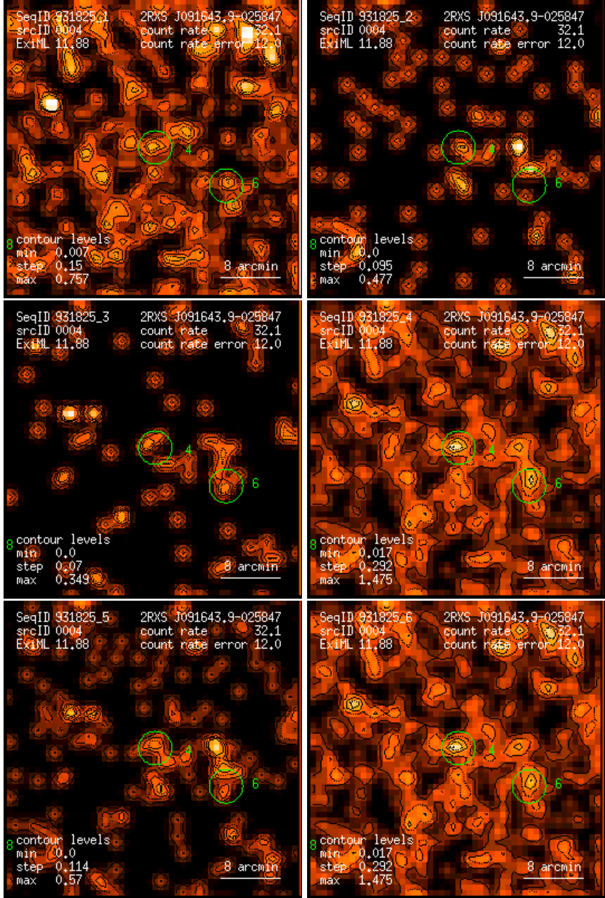
Figure 4: RASS 931825: detection 0004: band rate images, Gaussian filter: (1) PSPC channels 11 – 41, (2) 52 – 90, (3) 91 – 201, (4) 11 – 235, (5) 52 – 201, (6) 11 – 201. Broad band rates in counts/ks. Band rate contour levels in counts/ks/arcmin 2 .
