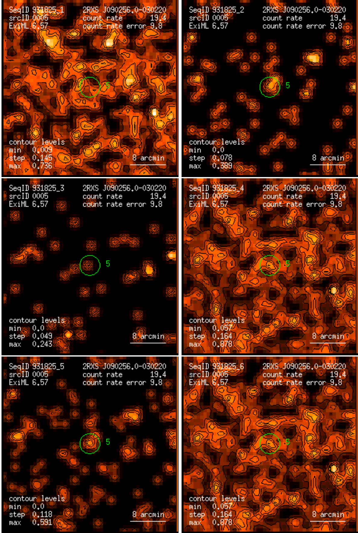
Figure 5: RASS 931825: detection 0005: band rate images, Gaussian filter: (1) PSPC channels 11 – 41, (2) 52 – 90, (3) 91 – 201, (4) 11 – 235, (5) 52 – 201, (6) 11 – 201. Broad band rates in counts/ks. Band rate contour levels in counts/ks/arcmin 2 .
