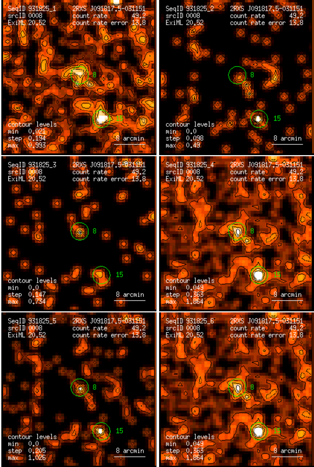
Figure 8: RASS 931825: detection 0008: band rate images, Gaussian filter: (1) PSPC channels 11 – 41, (2) 52 – 90, (3) 91 – 201, (4) 11 – 235, (5) 52 – 201, (6) 11 – 201. Broad band rates in counts/ks. Band rate contour levels in counts/ks/arcmin 2 .
