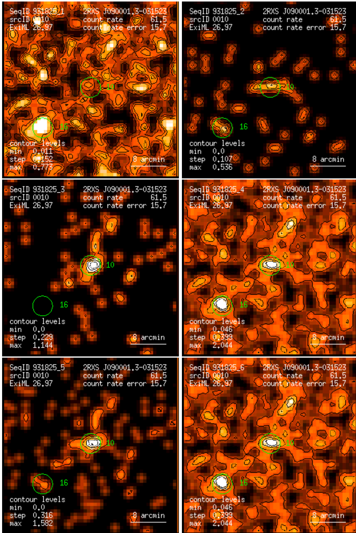
Figure 10: RASS 931825: detection 0010: band rate images, Gaussian filter: (1) PSPC channels 11 – 41, (2) 52 – 90, (3) 91 – 201, (4) 11 – 235, (5) 52 – 201, (6) 11 – 201. Broad band rates in counts/ks. Band rate contour levels in counts/ks/arcmin 2 .
