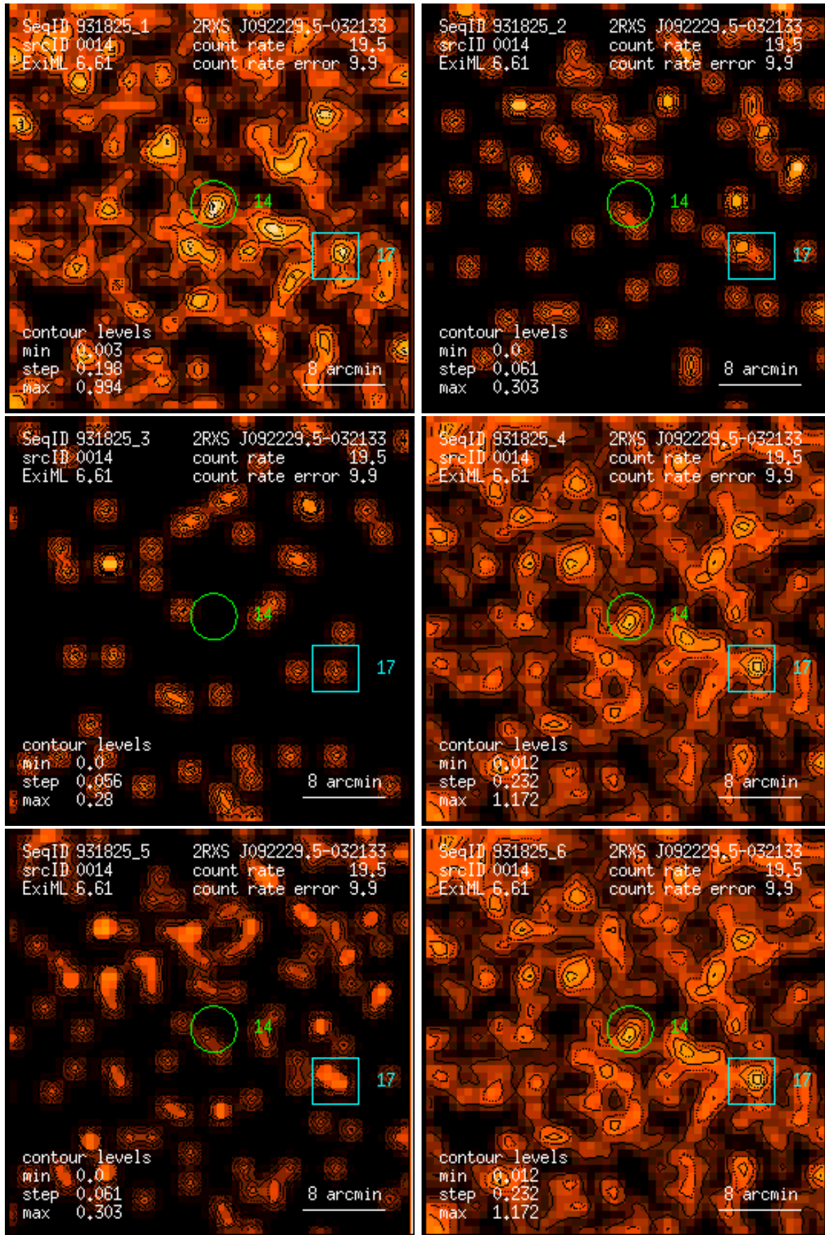
Figure 14: RASS 931825: detection 0014: band rate images, Gaussian filter: (1) PSPC channels 11 – 41, (2) 52 – 90, (3) 91 – 201, (4) 11 – 235, (5) 52 – 201, (6) 11 – 201. Broad band rates in counts/ks. Band rate contour levels in counts/ks/arcmin 2 .
