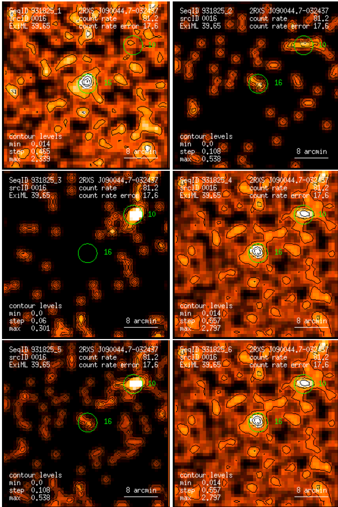
Figure 16: RASS 931825: detection 0016: band rate images, Gaussian filter: (1) PSPC channels 11 – 41, (2) 52 – 90, (3) 91 – 201, (4) 11 – 235, (5) 52 – 201, (6) 11 – 201. Broad band rates in counts/ks. Band rate contour levels in counts/ks/arcmin 2 .
