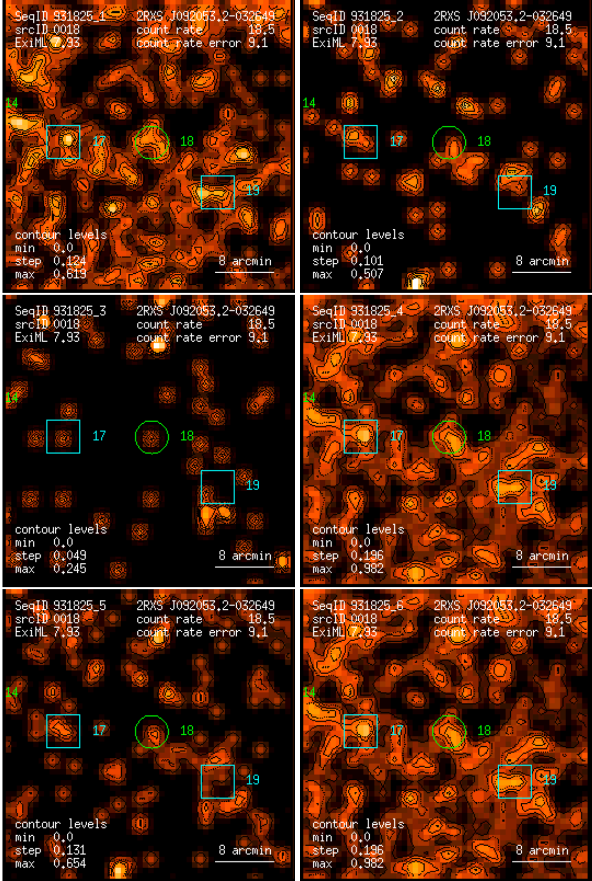
Figure 18: RASS 931825: detection 0018: band rate images, Gaussian filter: (1) PSPC channels 11 – 41, (2) 52 – 90, (3) 91 – 201, (4) 11 – 235, (5) 52 – 201, (6) 11 – 201. Broad band rates in counts/ks. Band rate contour levels in counts/ks/arcmin 2 .
