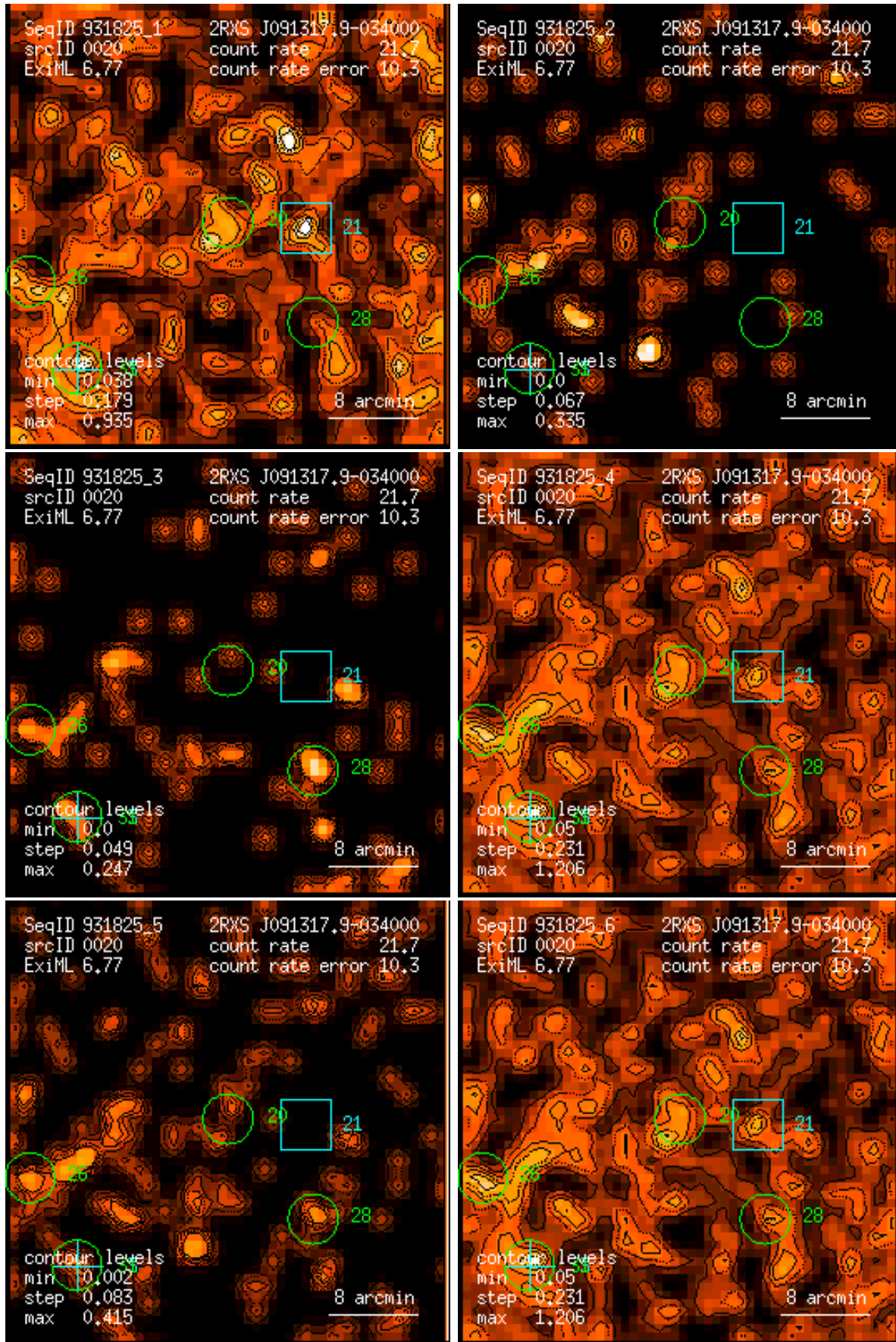
Figure 20: RASS 931825: detection 0020: band rate images, Gaussian filter: (1) PSPC channels 11 – 41, (2) 52 – 90, (3) 91 – 201, (4) 11 – 235, (5) 52 – 201, (6) 11 – 201. Broad band rates in counts/ks. Band rate contour levels in counts/ks/arcmin 2 .
