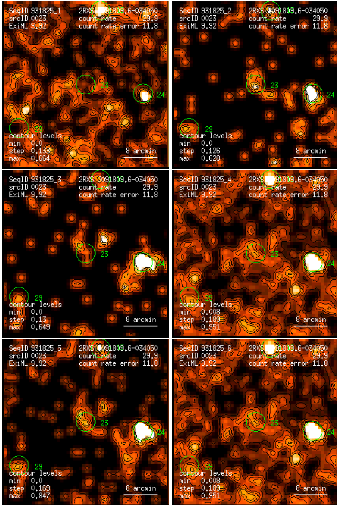
Figure 23: RASS 931825: detection 0023: band rate images, Gaussian filter: (1) PSPC channels 11 – 41, (2) 52 – 90, (3) 91 – 201, (4) 11 – 235, (5) 52 – 201, (6) 11 – 201. Broad band rates in counts/ks. Band rate contour levels in counts/ks/arcmin 2 .
