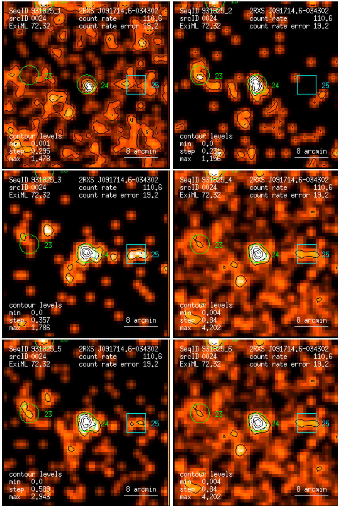
Figure 24: RASS 931825: detection 0024: band rate images, Gaussian filter: (1) PSPC channels 11 – 41, (2) 52 – 90, (3) 91 – 201, (4) 11 – 235, (5) 52 – 201, (6) 11 – 201. Broad band rates in counts/ks. Band rate contour levels in counts/ks/arcmin 2 .
