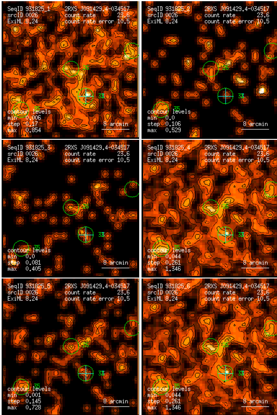
Figure 26: RASS 931825: detection 0026: band rate images, Gaussian filter: (1) PSPC channels 11 – 41, (2) 52 – 90, (3) 91 – 201, (4) 11 – 235, (5) 52 – 201, (6) 11 – 201. Broad band rates in counts/ks. Band rate contour levels in counts/ks/arcmin 2 .
