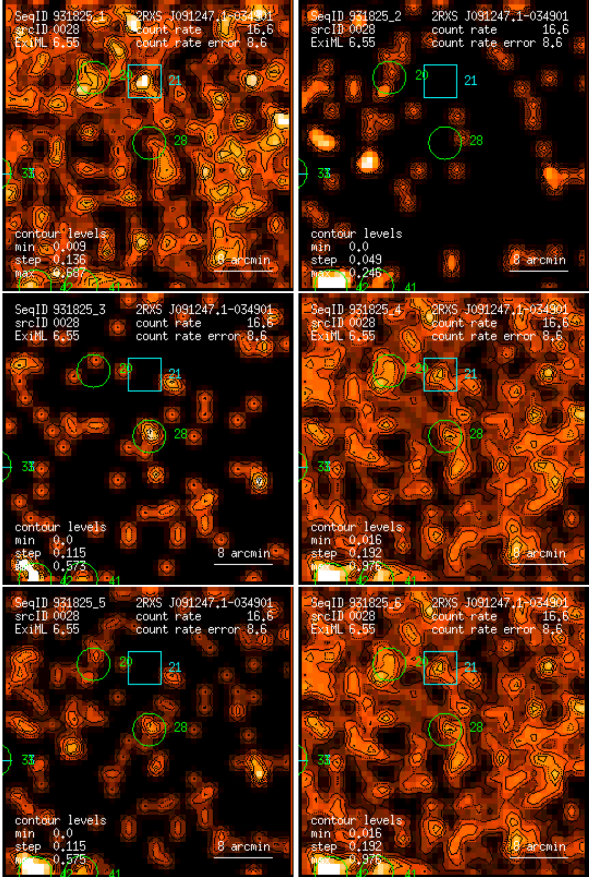
Figure 28: RASS 931825: detection 0028: band rate images, Gaussian filter: (1) PSPC channels 11 – 41, (2) 52 – 90, (3) 91 – 201, (4) 11 – 235, (5) 52 – 201, (6) 11 – 201. Broad band rates in counts/ks. Band rate contour levels in counts/ks/arcmin 2 .
