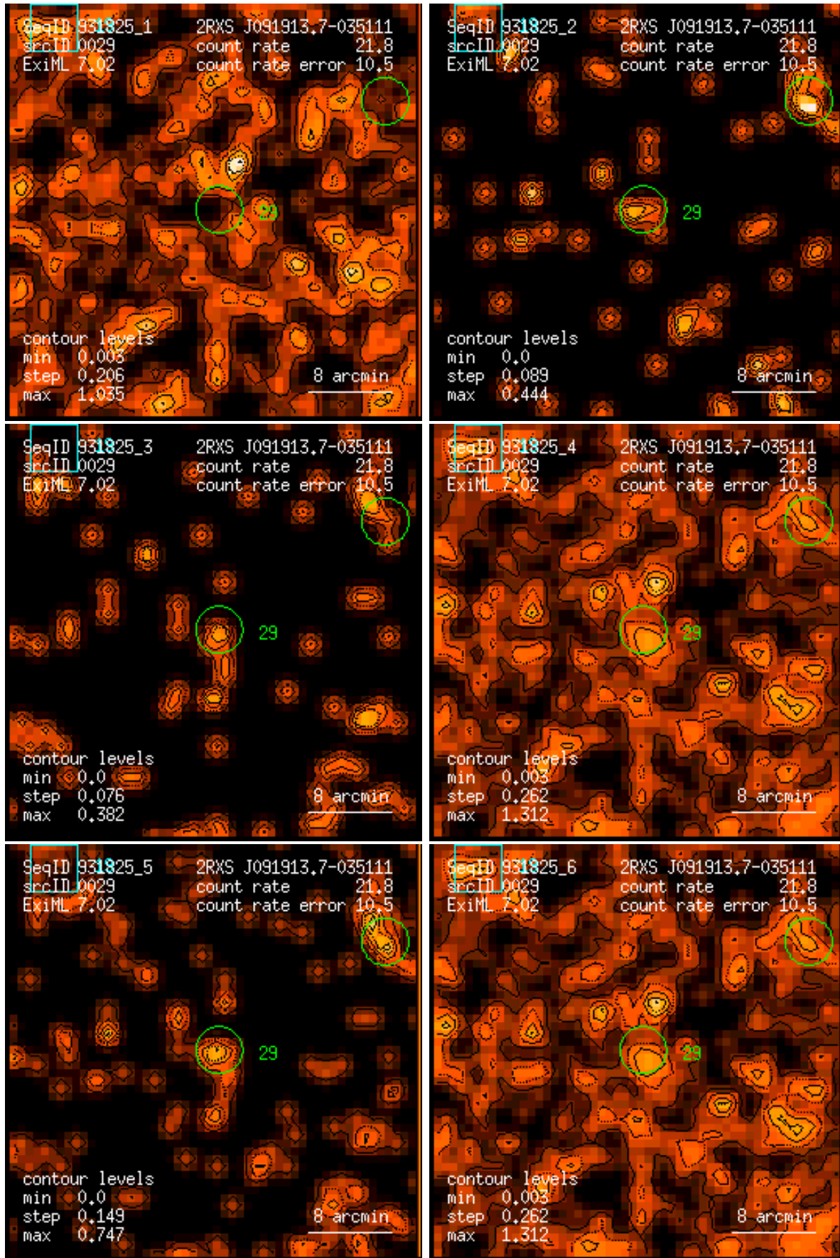
Figure 29: RASS 931825: detection 0029: band rate images, Gaussian filter: (1) PSPC channels 11 – 41, (2) 52 – 90, (3) 91 – 201, (4) 11 – 235, (5) 52 – 201, (6) 11 – 201. Broad band rates in counts/ks. Band rate contour levels in counts/ks/arcmin 2 .
