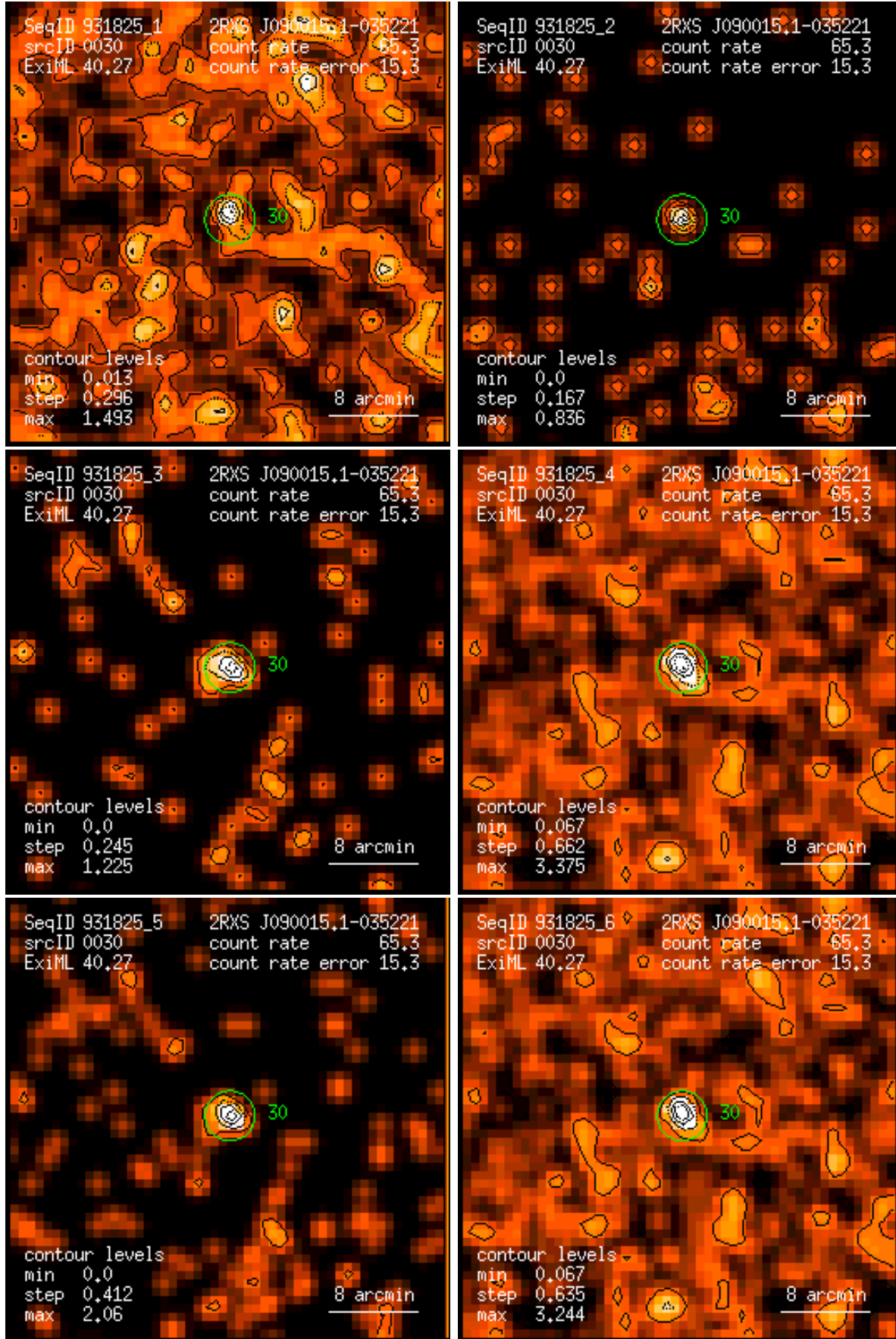
Figure 30: RASS 931825: detection 0030: band rate images, Gaussian filter: (1) PSPC channels 11 – 41, (2) 52 – 90, (3) 91 – 201, (4) 11 – 235, (5) 52 – 201, (6) 11 – 201. Broad band rates in counts/ks. Band rate contour levels in counts/ks/arcmin 2 .
