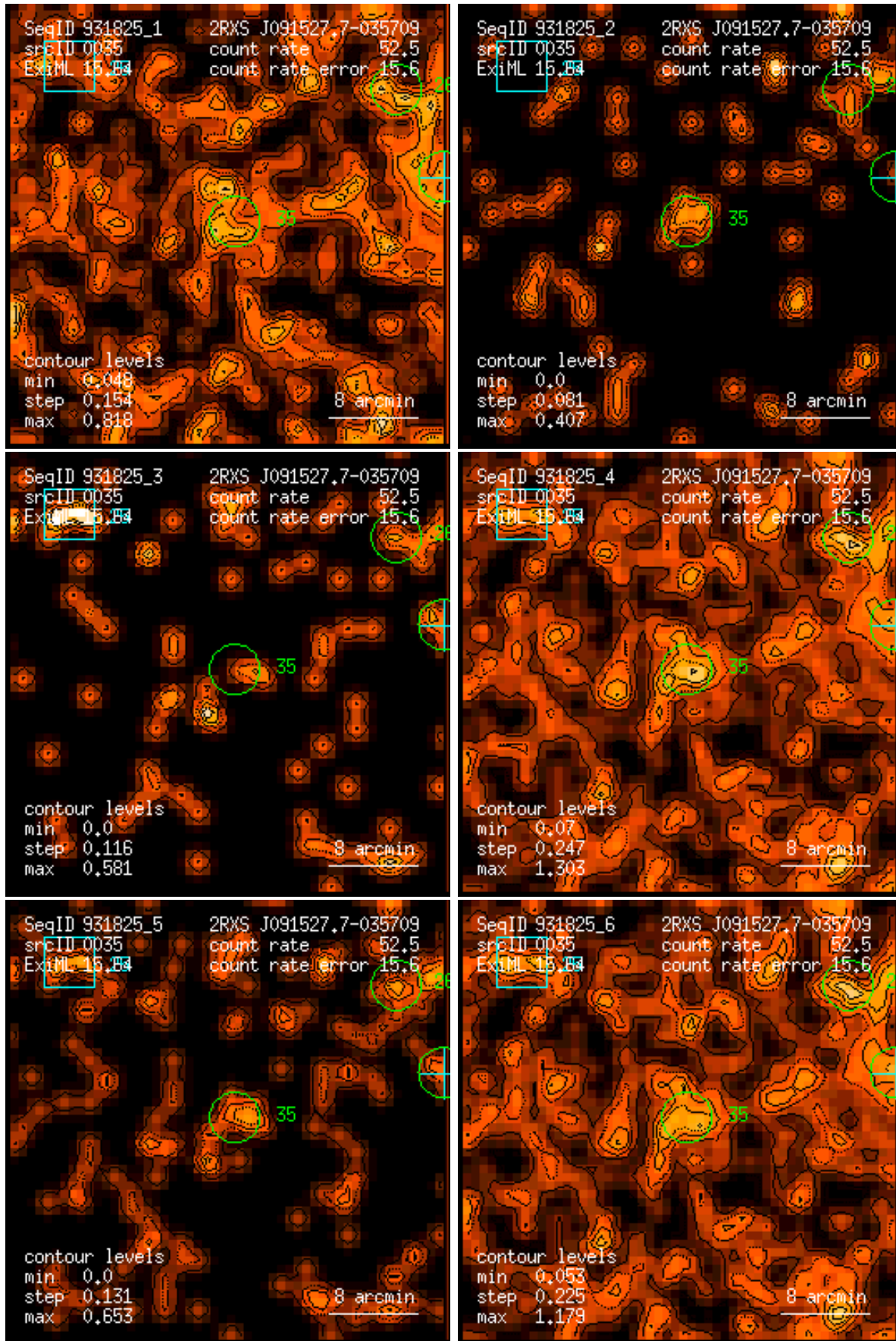
Figure 35: RASS 931825: detection 0035: band rate images, Gaussian filter: (1) PSPC channels 11 – 41, (2) 52 – 90, (3) 91 – 201, (4) 11 – 235, (5) 52 – 201, (6) 11 – 201. Broad band rates in counts/ks. Band rate contour levels in counts/ks/arcmin 2 .
