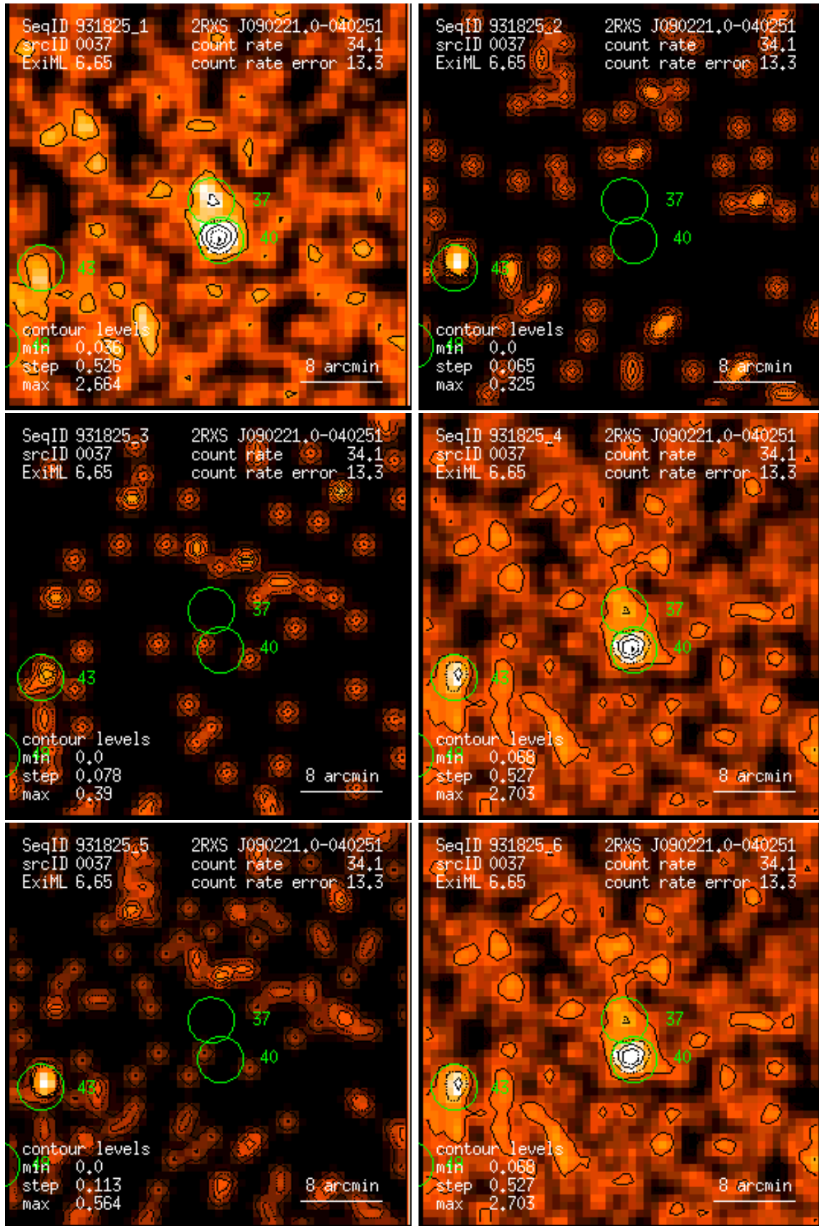
Figure 37: RASS 931825: detection 0037: band rate images, Gaussian filter: (1) PSPC channels 11 – 41, (2) 52 – 90, (3) 91 – 201, (4) 11 – 235, (5) 52 – 201, (6) 11 – 201. Broad band rates in counts/ks. Band rate contour levels in counts/ks/arcmin 2 .
