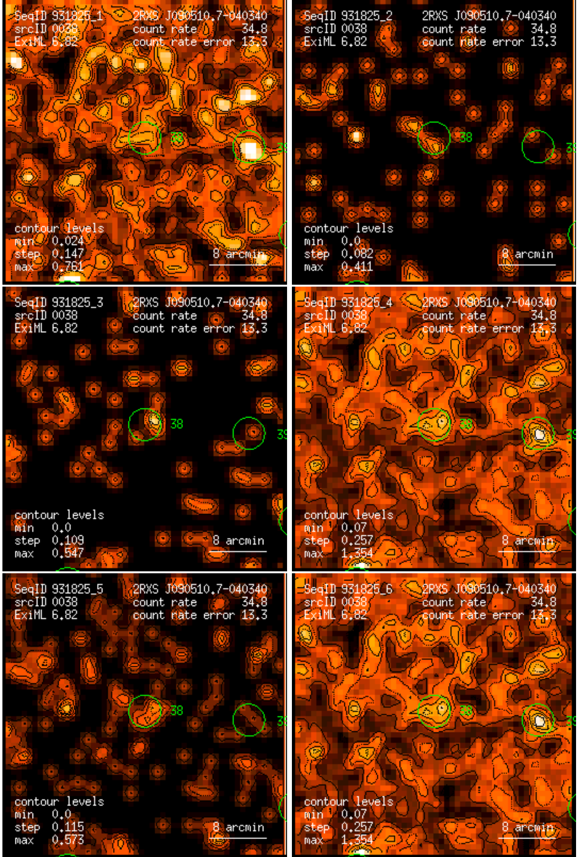
Figure 38: RASS 931825: detection 0038: band rate images, Gaussian filter: (1) PSPC channels 11 – 41, (2) 52 – 90, (3) 91 – 201, (4) 11 – 235, (5) 52 – 201, (6) 11 – 201. Broad band rates in counts/ks. Band rate contour levels in counts/ks/arcmin 2 .
