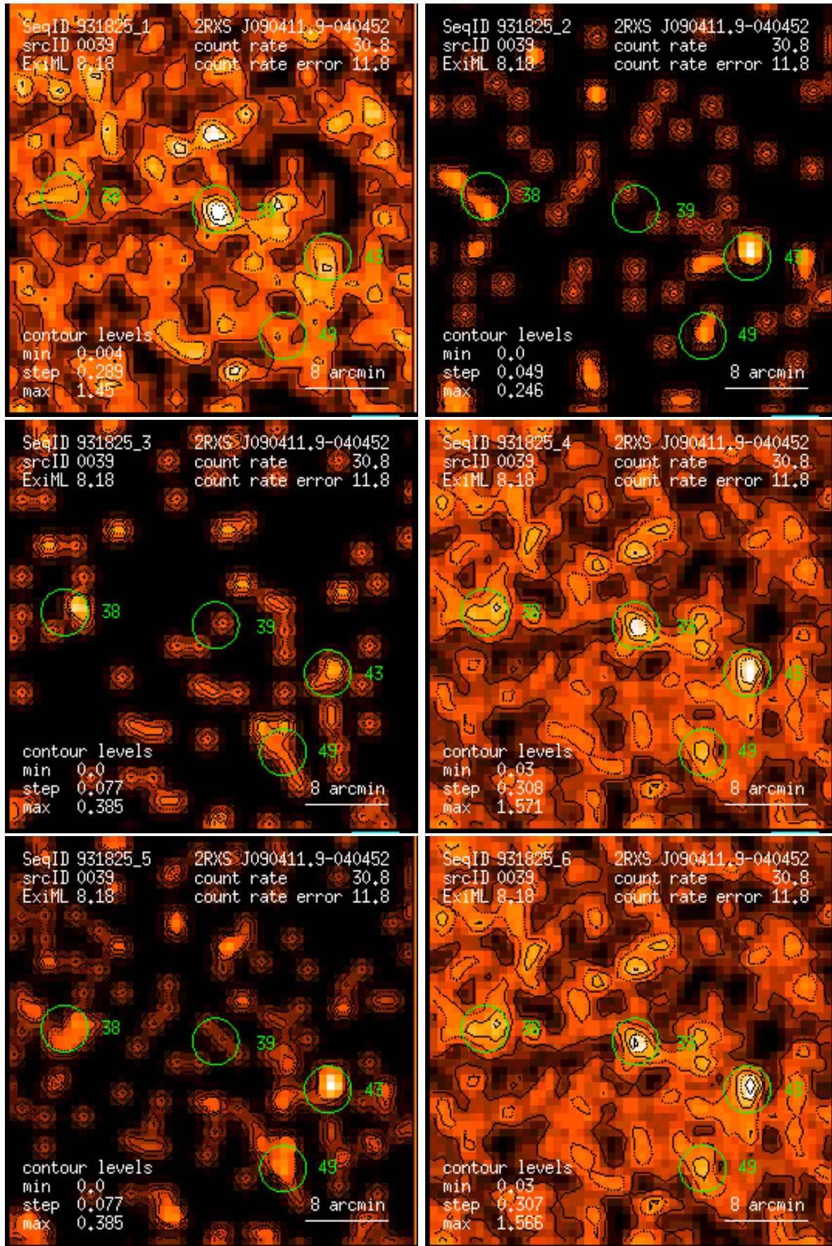
Figure 39: RASS 931825: detection 0039: band rate images, Gaussian filter: (1) PSPC channels 11 – 41, (2) 52 – 90, (3) 91 – 201, (4) 11 – 235, (5) 52 – 201, (6) 11 – 201. Broad band rates in counts/ks. Band rate contour levels in counts/ks/arcmin 2 .
