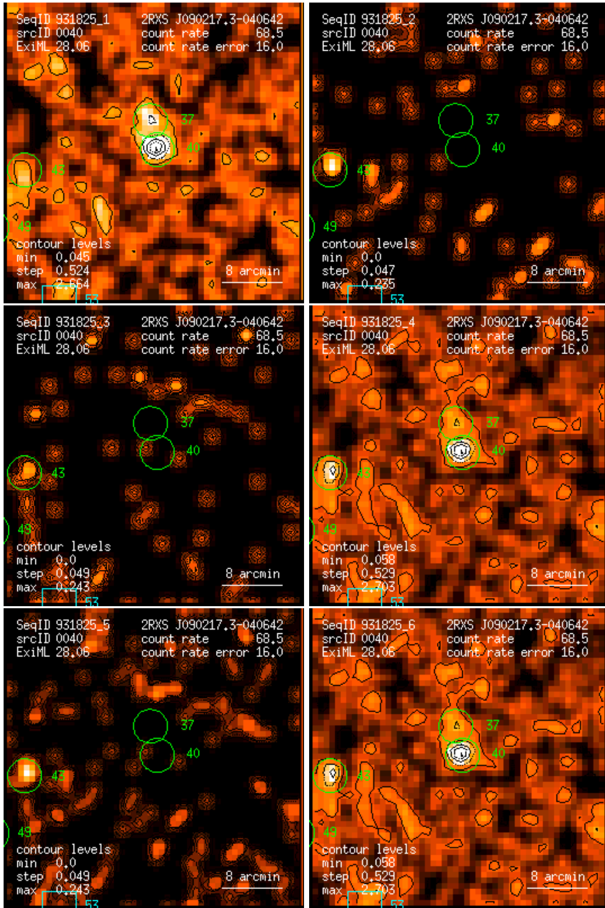
Figure 40: RASS 931825: detection 0040: band rate images, Gaussian filter: (1) PSPC channels 11 – 41, (2) 52 – 90, (3) 91 – 201, (4) 11 – 235, (5) 52 – 201, (6) 11 – 201. Broad band rates in counts/ks. Band rate contour levels in counts/ks/arcmin 2 .
