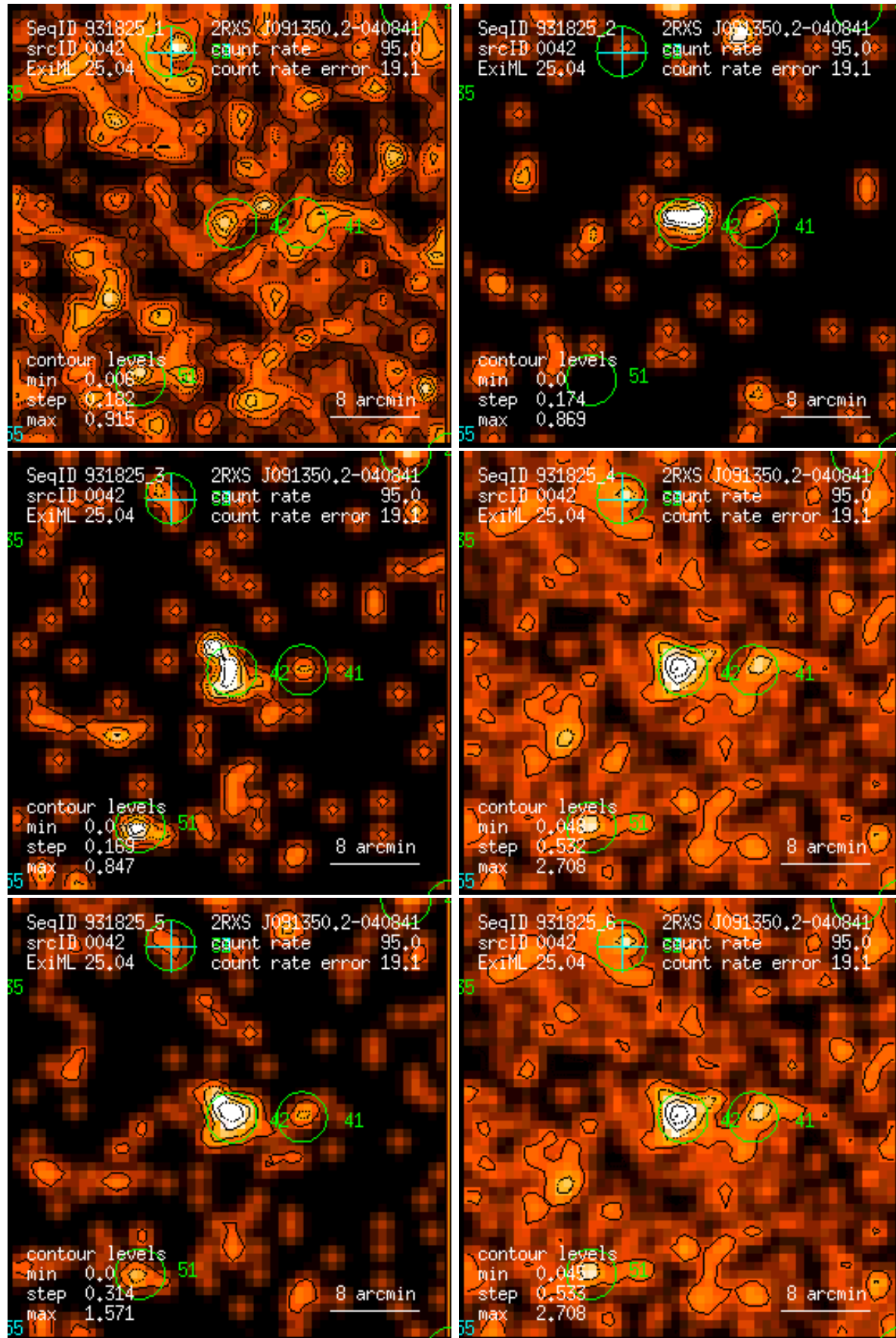
Figure 42: RASS 931825: detection 0042: band rate images, Gaussian filter: (1) PSPC channels 11 – 41, (2) 52 – 90, (3) 91 – 201, (4) 11 – 235, (5) 52 – 201, (6) 11 – 201. Broad band rates in counts/ks. Band rate contour levels in counts/ks/arcmin 2 .
