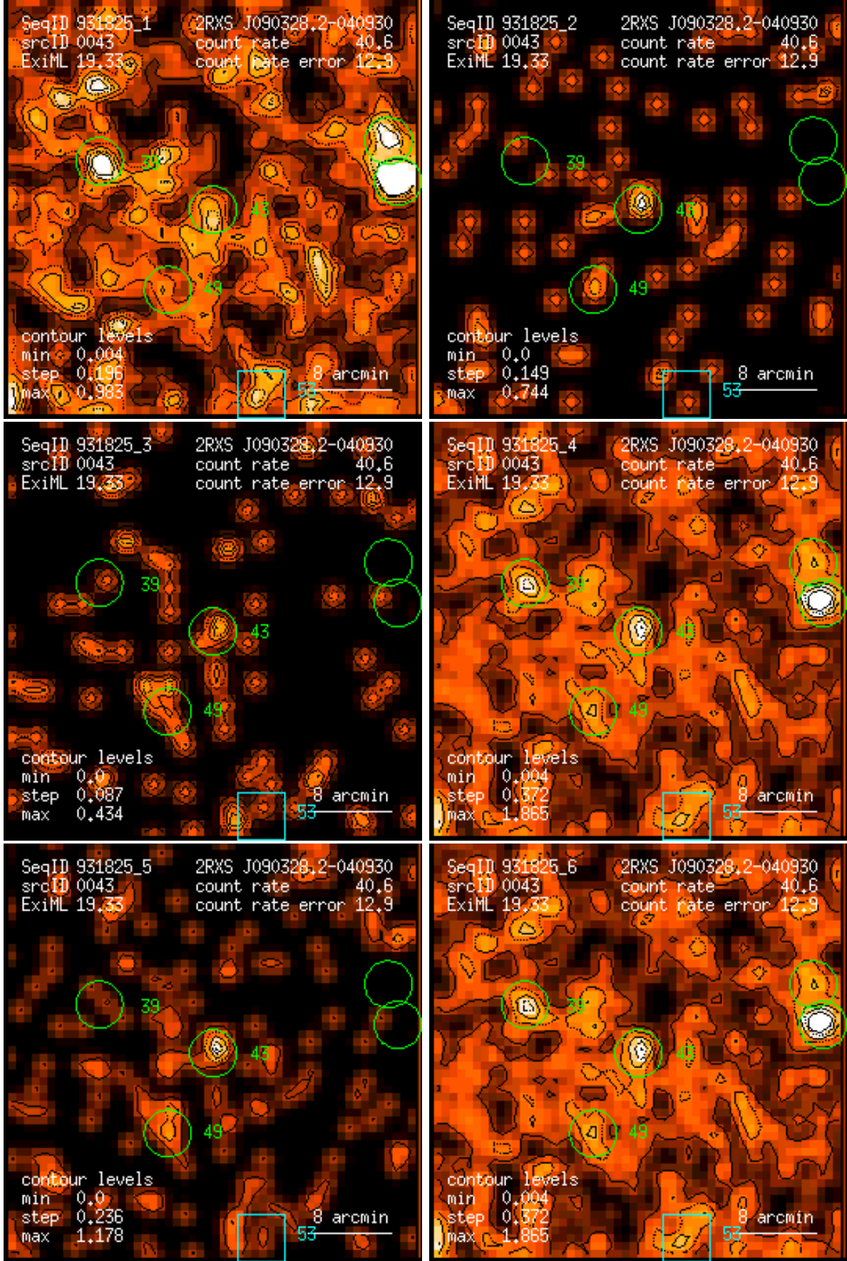
Figure 43: RASS 931825: detection 0043: band rate images, Gaussian filter: (1) PSPC channels 11 – 41, (2) 52 – 90, (3) 91 – 201, (4) 11 – 235, (5) 52 – 201, (6) 11 – 201. Broad band rates in counts/ks. Band rate contour levels in counts/ks/arcmin 2 .
