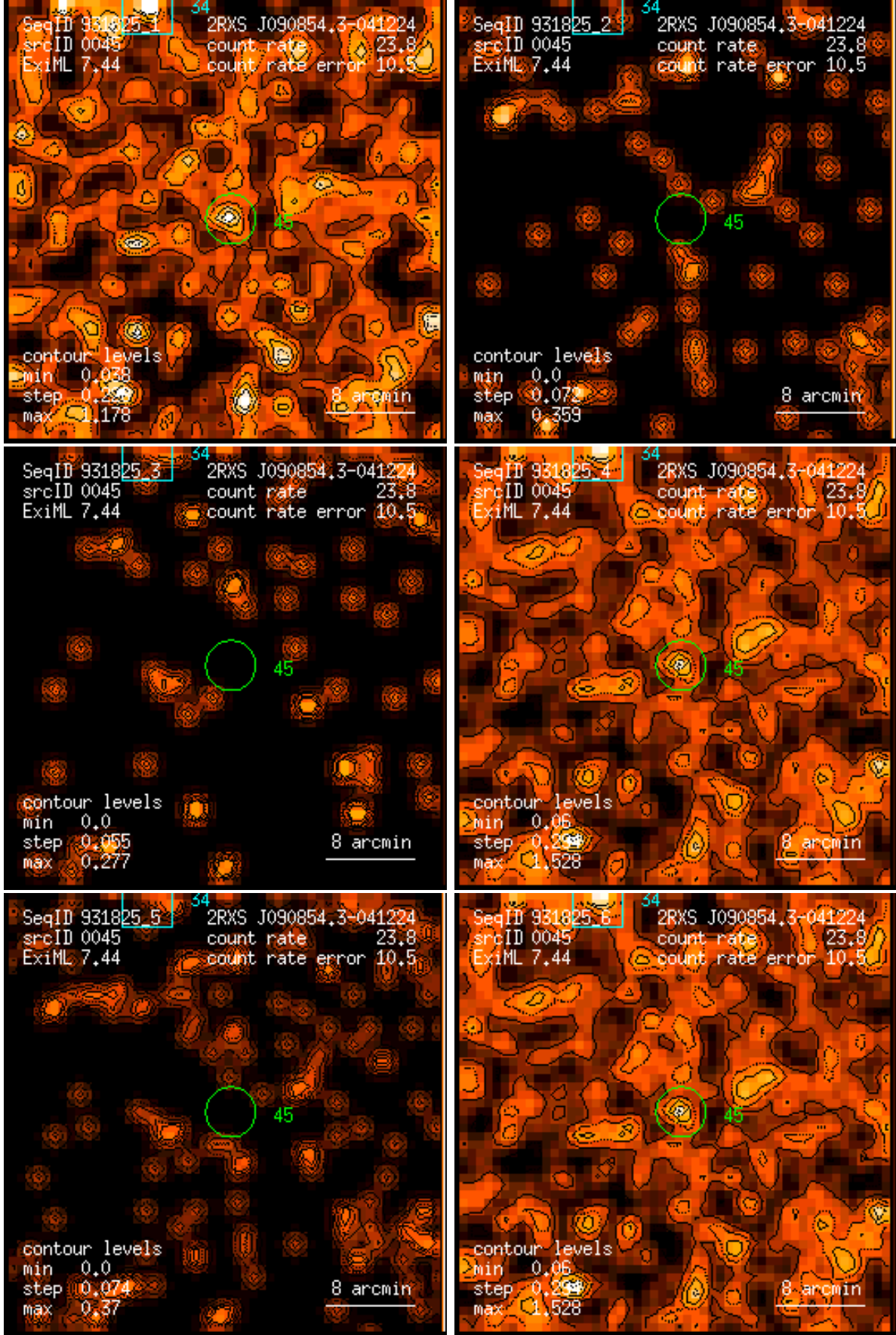
Figure 45: RASS 931825: detection 0045: band rate images, Gaussian filter: (1) PSPC channels 11 – 41, (2) 52 – 90, (3) 91 – 201, (4) 11 – 235, (5) 52 – 201, (6) 11 – 201. Broad band rates in counts/ks. Band rate contour levels in counts/ks/arcmin 2 .
