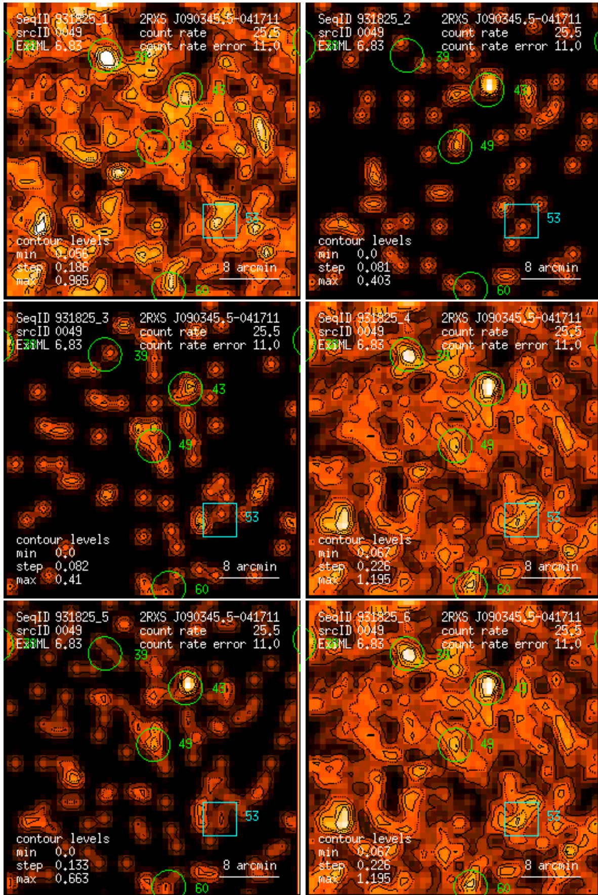
Figure 49: RASS 931825: detection 0049: band rate images, Gaussian filter: (1) PSPC channels 11 – 41, (2) 52 – 90, (3) 91 – 201, (4) 11 – 235, (5) 52 – 201, (6) 11 – 201. Broad band rates in counts/ks. Band rate contour levels in counts/ks/arcmin 2 .
