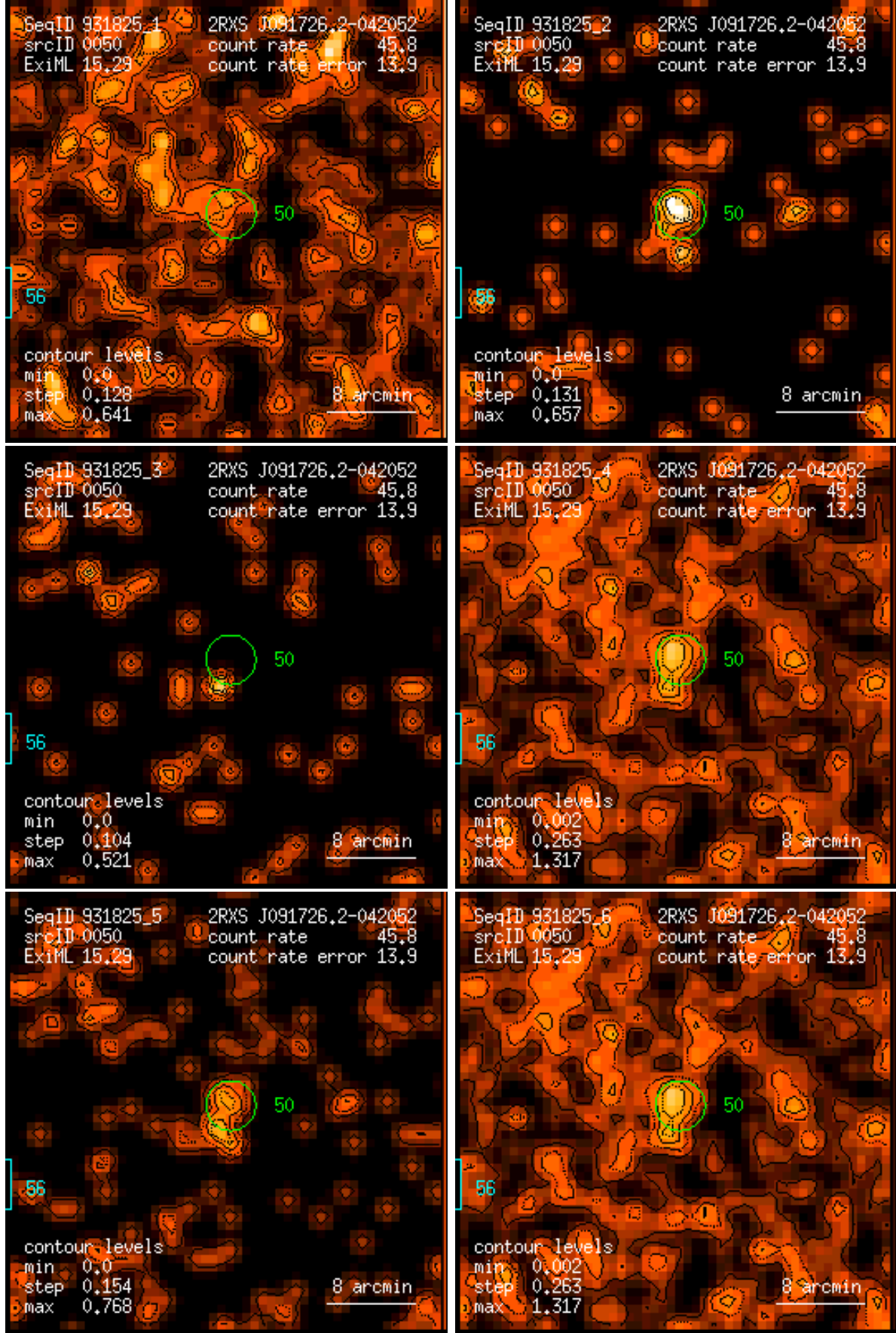
Figure 50: RASS 931825: detection 0050: band rate images, Gaussian filter: (1) PSPC channels 11 – 41, (2) 52 – 90, (3) 91 – 201, (4) 11 – 235, (5) 52 – 201, (6) 11 – 201. Broad band rates in counts/ks. Band rate contour levels in counts/ks/arcmin 2 .
