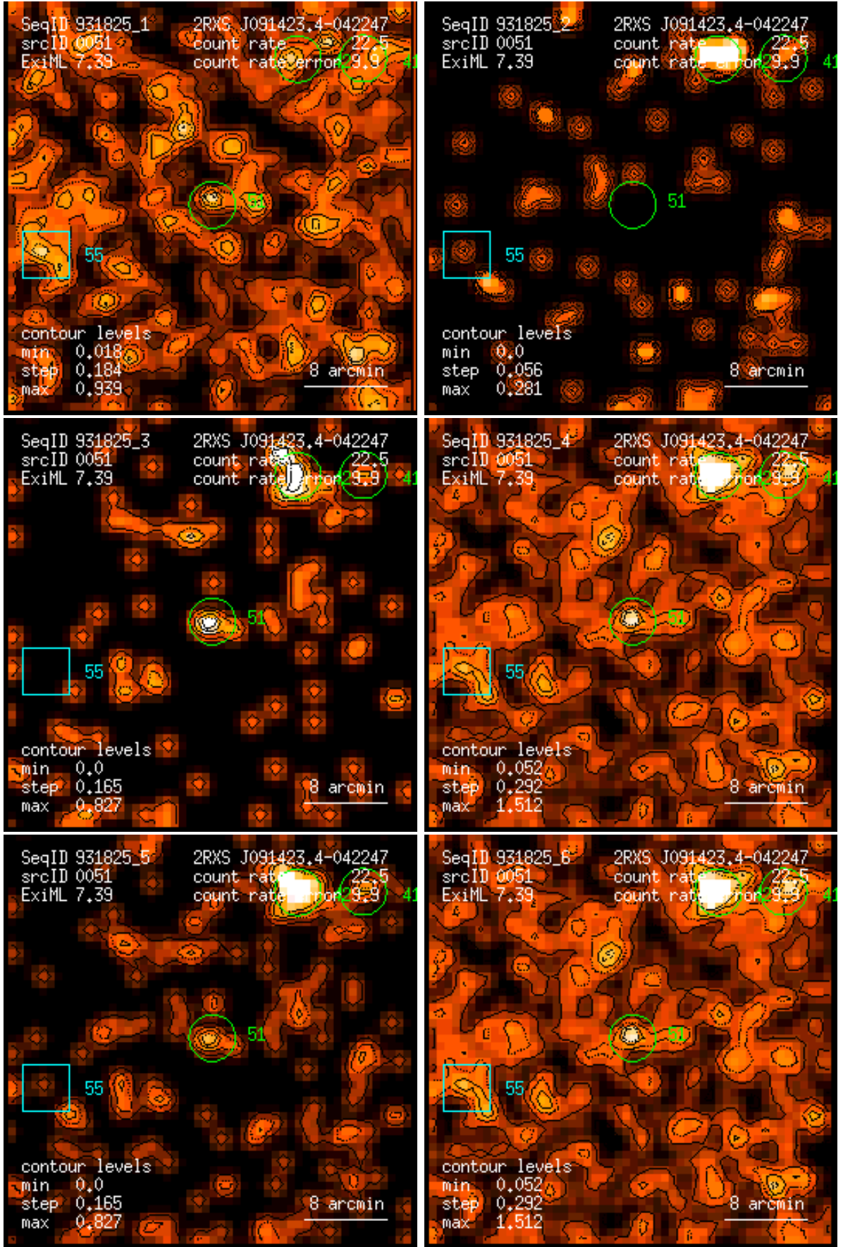
Figure 51: RASS 931825: detection 0051: band rate images, Gaussian filter: (1) PSPC channels 11 – 41, (2) 52 – 90, (3) 91 – 201, (4) 11 – 235, (5) 52 – 201, (6) 11 – 201. Broad band rates in counts/ks. Band rate contour levels in counts/ks/arcmin 2 .
