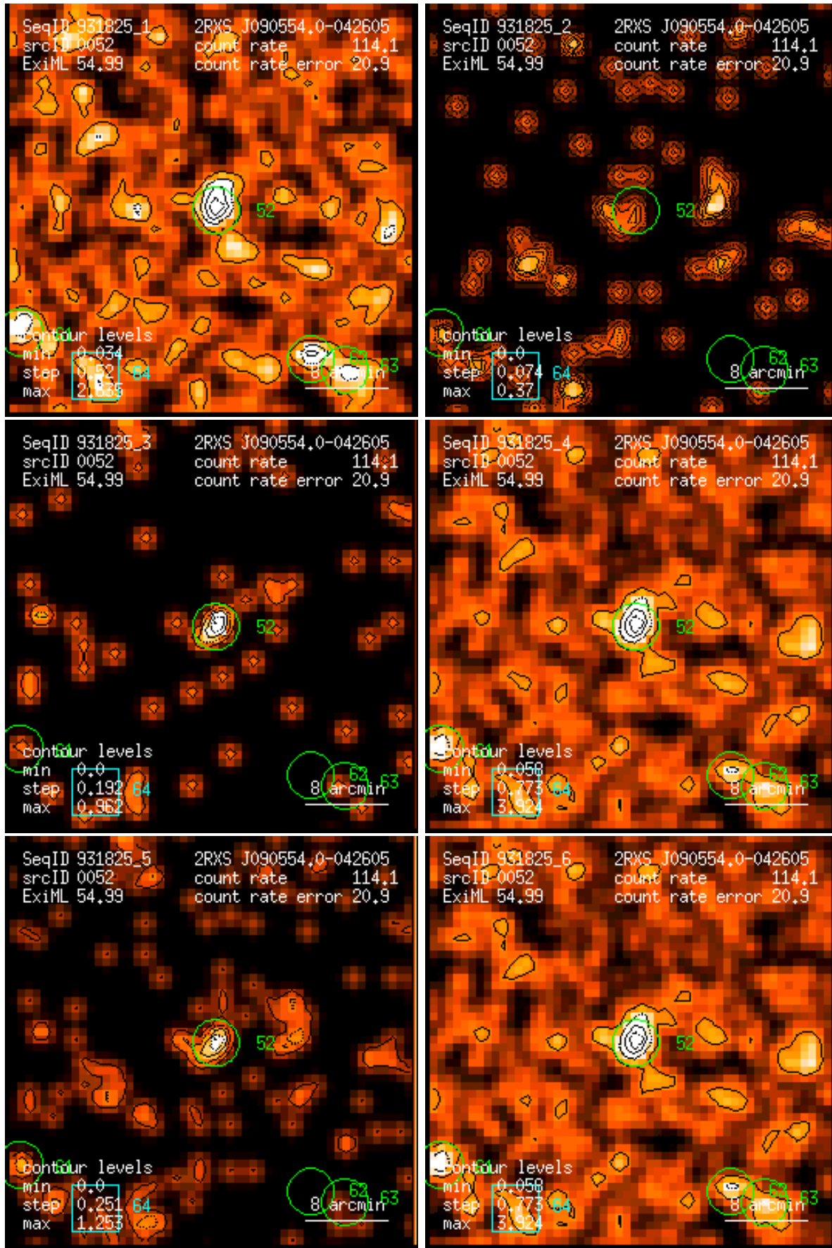
Figure 52: RASS 931825: detection 0052: band rate images, Gaussian filter: (1) PSPC channels 11 – 41, (2) 52 – 90, (3) 91 – 201, (4) 11 – 235, (5) 52 – 201, (6) 11 – 201. Broad band rates in counts/ks. Band rate contour levels in counts/ks/arcmin 2 .
