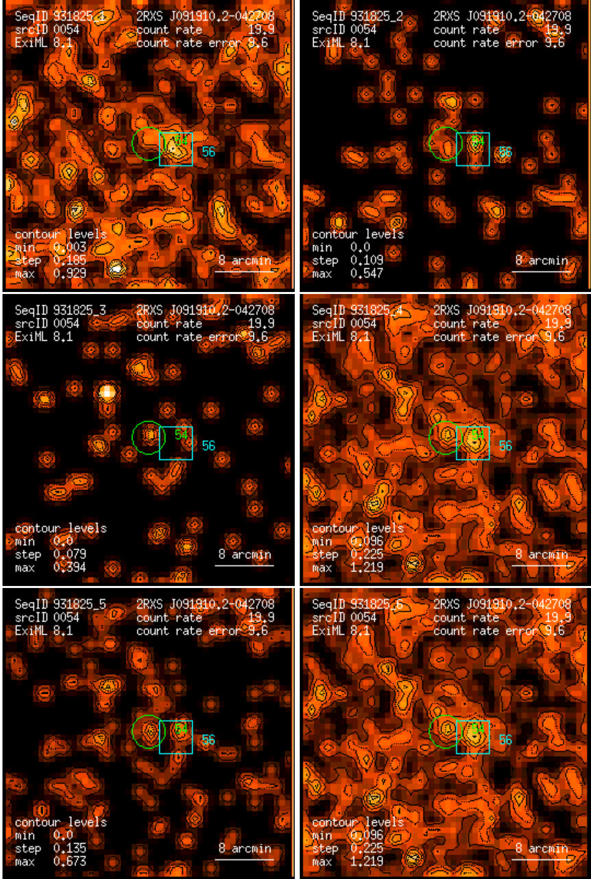
Figure 54: RASS 931825: detection 0054: band rate images, Gaussian filter: (1) PSPC channels 11 – 41, (2) 52 – 90, (3) 91 – 201, (4) 11 – 235, (5) 52 – 201, (6) 11 – 201. Broad band rates in counts/ks. Band rate contour levels in counts/ks/arcmin 2 .
