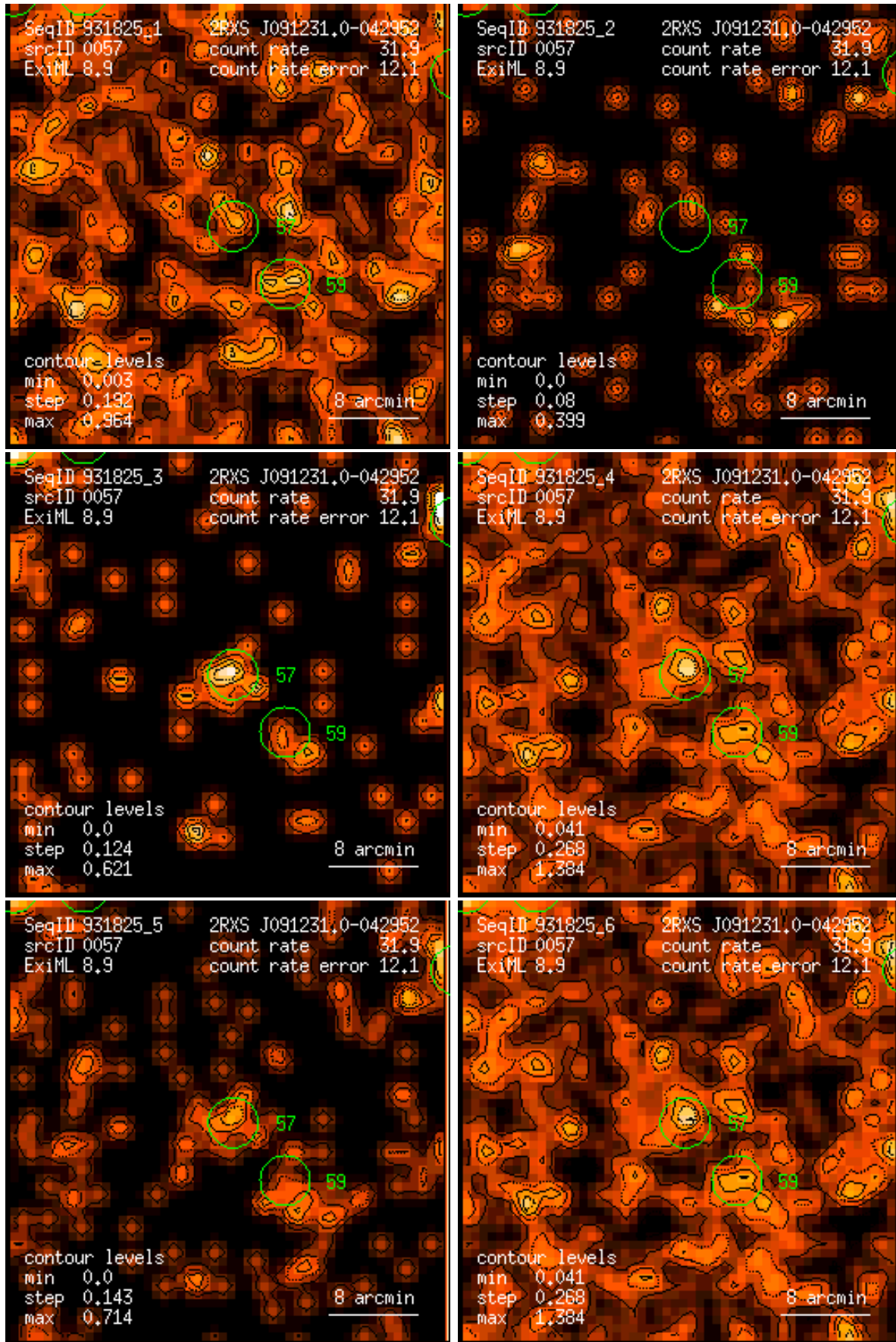
Figure 57: RASS 931825: detection 0057: band rate images, Gaussian filter: (1) PSPC channels 11 – 41, (2) 52 – 90, (3) 91 – 201, (4) 11 – 235, (5) 52 – 201, (6) 11 – 201. Broad band rates in counts/ks. Band rate contour levels in counts/ks/arcmin 2 .
