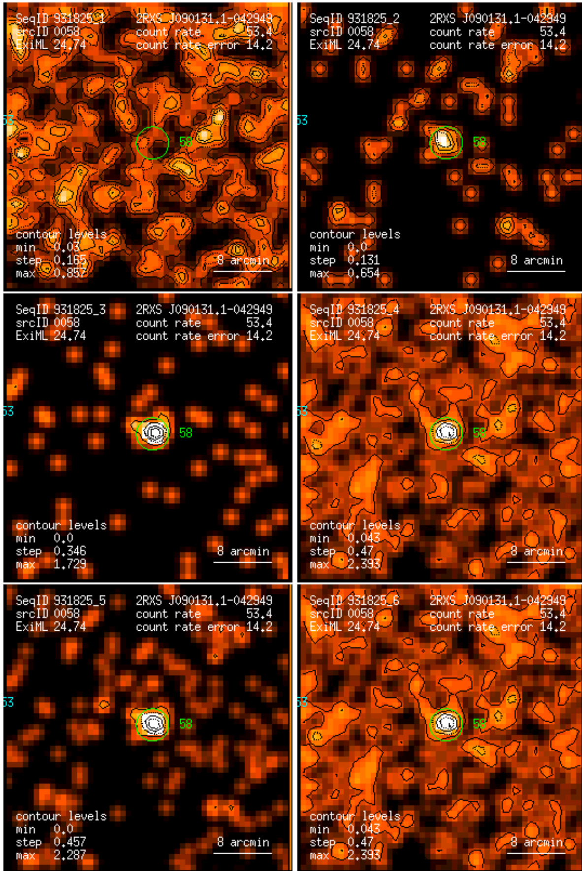
Figure 58: RASS 931825: detection 0058: band rate images, Gaussian filter: (1) PSPC channels 11 – 41, (2) 52 – 90, (3) 91 – 201, (4) 11 – 235, (5) 52 – 201, (6) 11 – 201. Broad band rates in counts/ks. Band rate contour levels in counts/ks/arcmin 2 .
