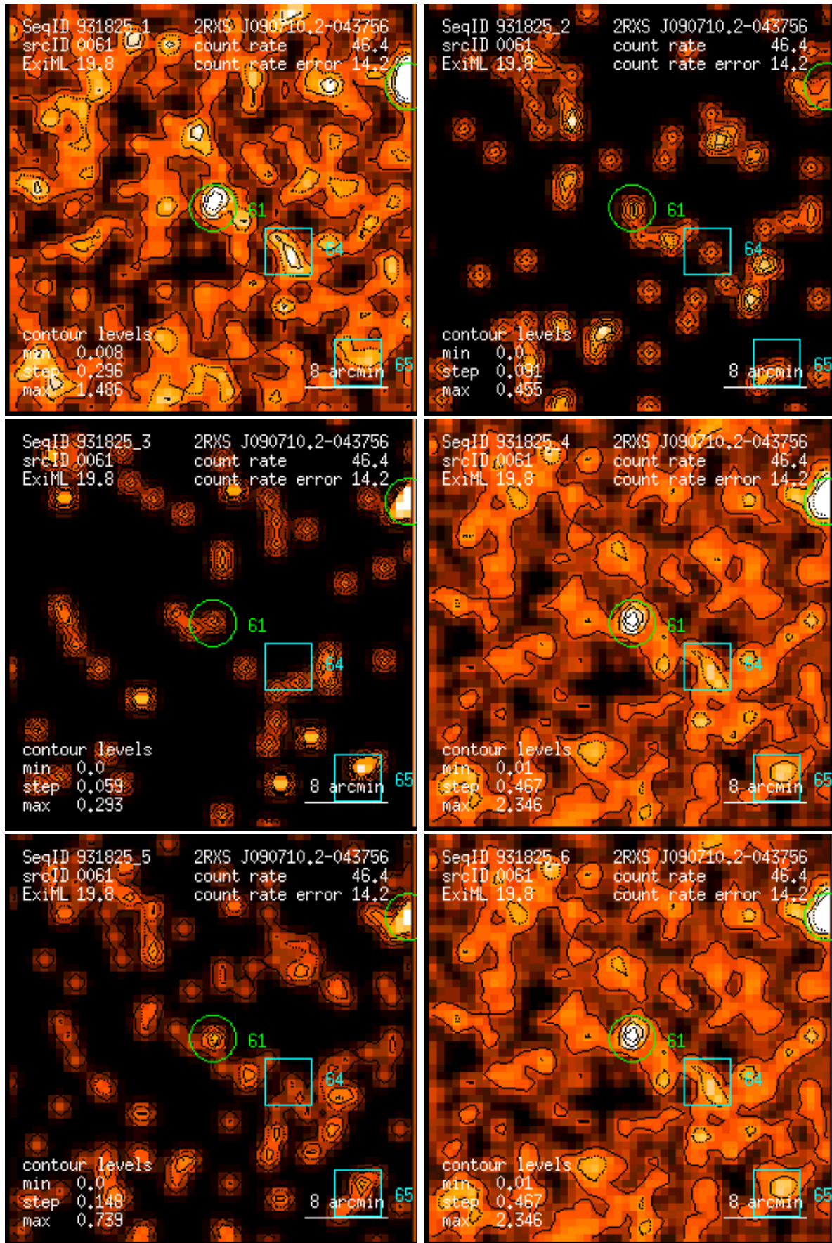
Figure 61: RASS 931825: detection 0061: band rate images, Gaussian filter: (1) PSPC channels 11 – 41, (2) 52 – 90, (3) 91 – 201, (4) 11 – 235, (5) 52 – 201, (6) 11 – 201. Broad band rates in counts/ks. Band rate contour levels in counts/ks/arcmin 2 .
