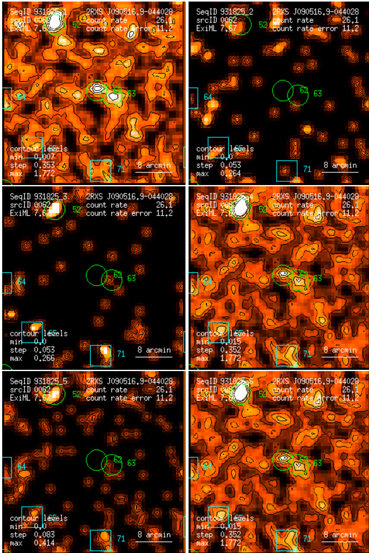
Figure 62: RASS 931825: detection 0062: band rate images, Gaussian filter: (1) PSPC channels 11 – 41, (2) 52 – 90, (3) 91 – 201, (4) 11 – 235, (5) 52 – 201, (6) 11 – 201. Broad band rates in counts/ks. Band rate contour levels in counts/ks/arcmin 2 .
