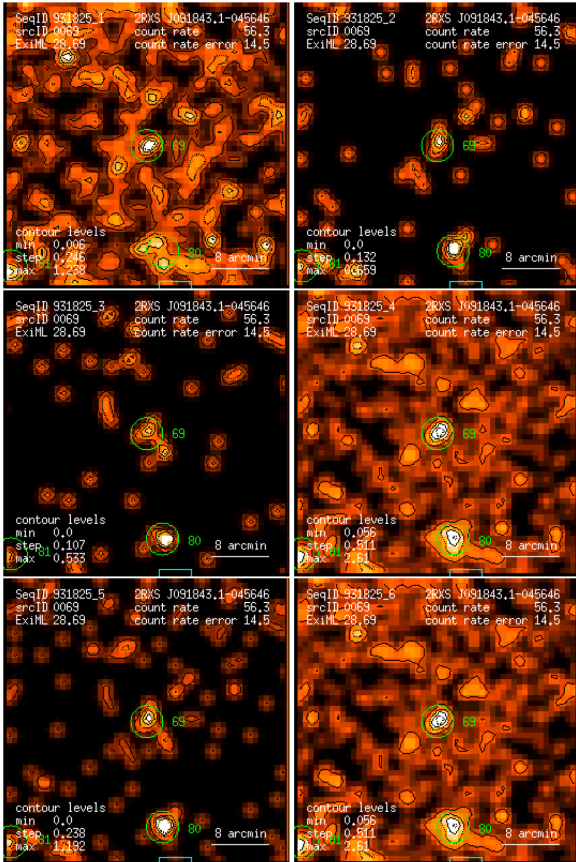
Figure 69: RASS 931825: detection 0069: band rate images, Gaussian filter: (1) PSPC channels 11 – 41, (2) 52 – 90, (3) 91 – 201, (4) 11 – 235, (5) 52 – 201, (6) 11 – 201. Broad band rates in counts/ks. Band rate contour levels in counts/ks/arcmin 2 .
