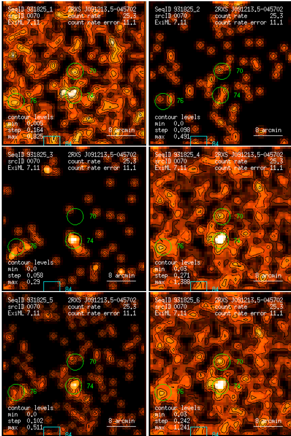
Figure 70: RASS 931825: detection 0070: band rate images, Gaussian filter: (1) PSPC channels 11 – 41, (2) 52 – 90, (3) 91 – 201, (4) 11 – 235, (5) 52 – 201, (6) 11 – 201. Broad band rates in counts/ks. Band rate contour levels in counts/ks/arcmin 2 .
