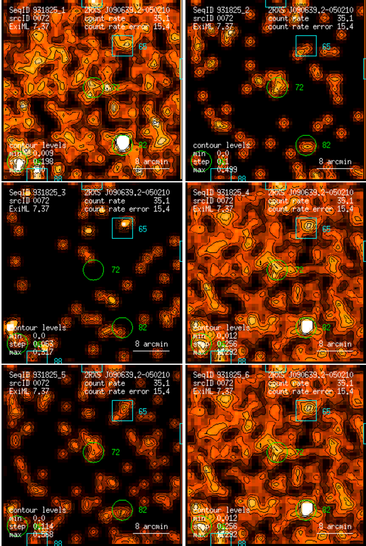
Figure 72: RASS 931825: detection 0072: band rate images, Gaussian filter: (1) PSPC channels 11 – 41, (2) 52 – 90, (3) 91 – 201, (4) 11 – 235, (5) 52 – 201, (6) 11 – 201. Broad band rates in counts/ks. Band rate contour levels in counts/ks/arcmin 2 .
