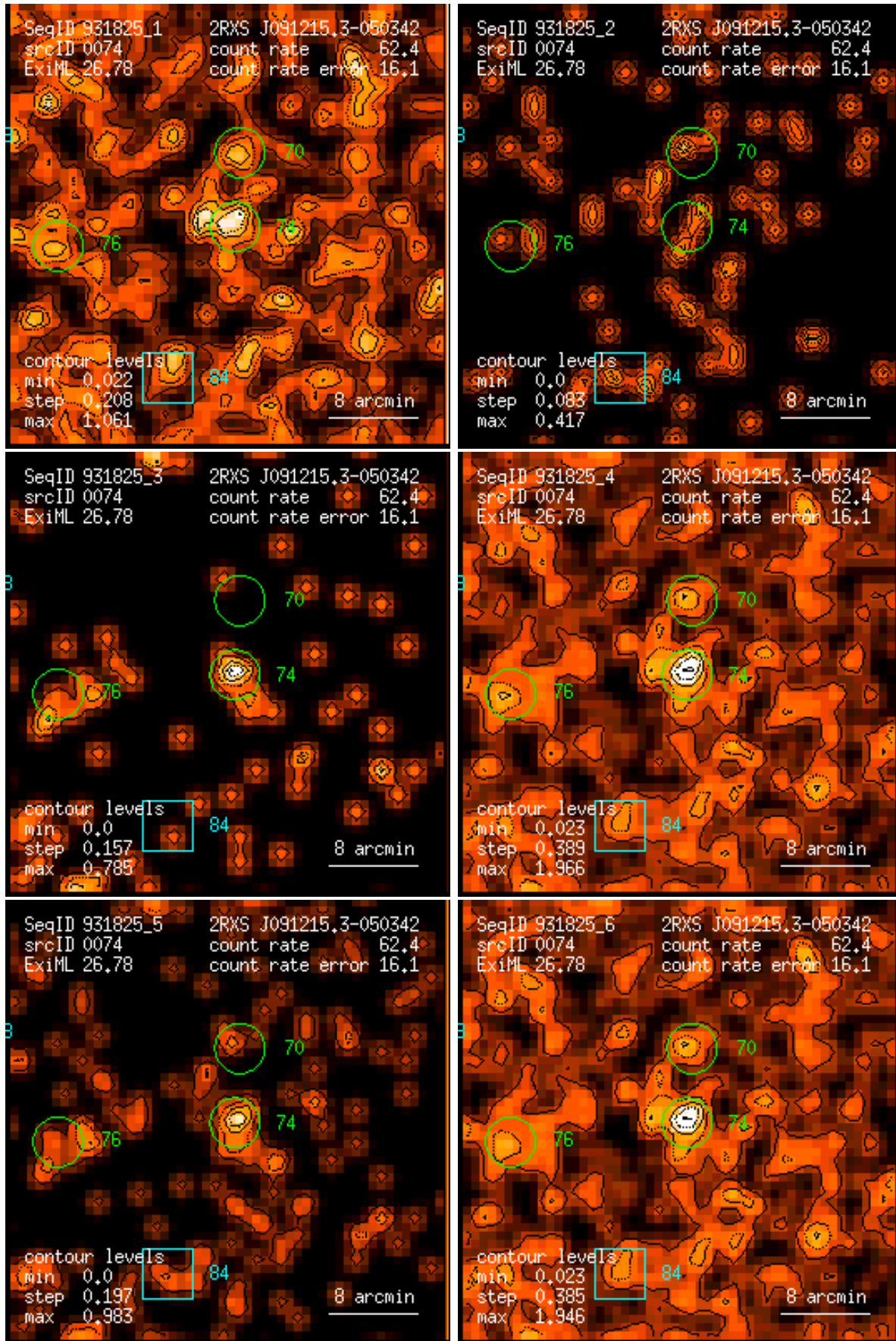
Figure 74: RASS 931825: detection 0074: band rate images, Gaussian filter: (1) PSPC channels 11 – 41, (2) 52 – 90, (3) 91 – 201, (4) 11 – 235, (5) 52 – 201, (6) 11 – 201. Broad band rates in counts/ks. Band rate contour levels in counts/ks/arcmin 2 .
