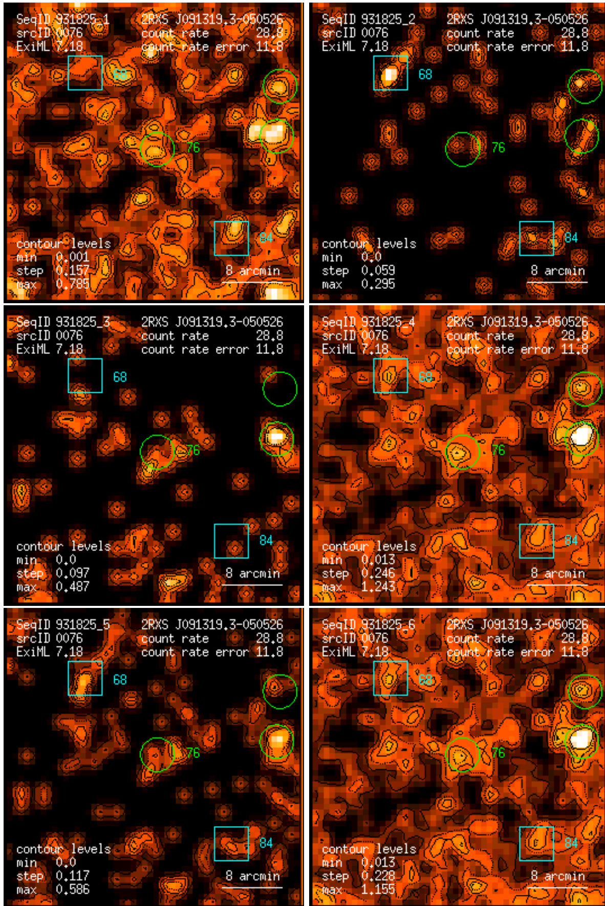
Figure 76: RASS 931825: detection 0076: band rate images, Gaussian filter: (1) PSPC channels 11 – 41, (2) 52 – 90, (3) 91 – 201, (4) 11 – 235, (5) 52 – 201, (6) 11 – 201. Broad band rates in counts/ks. Band rate contour levels in counts/ks/arcmin 2 .
