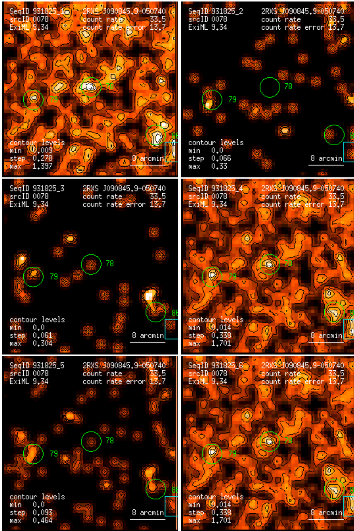
Figure 78: RASS 931825: detection 0078: band rate images, Gaussian filter: (1) PSPC channels 11 – 41, (2) 52 – 90, (3) 91 – 201, (4) 11 – 235, (5) 52 – 201, (6) 11 – 201. Broad band rates in counts/ks. Band rate contour levels in counts/ks/arcmin 2 .
