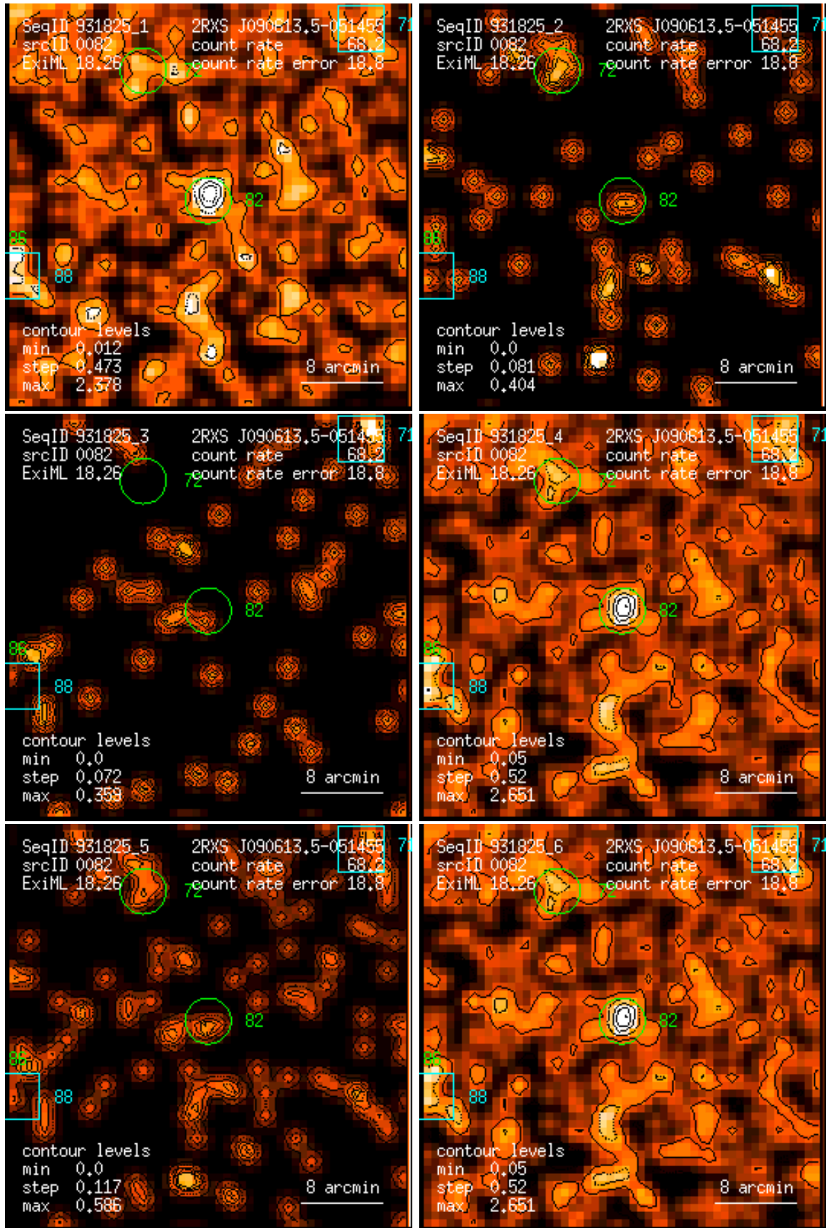
Figure 82: RASS 931825: detection 0082: band rate images, Gaussian filter: (1) PSPC channels 11 – 41, (2) 52 – 90, (3) 91 – 201, (4) 11 – 235, (5) 52 – 201, (6) 11 – 201. Broad band rates in counts/ks. Band rate contour levels in counts/ks/arcmin 2 .
