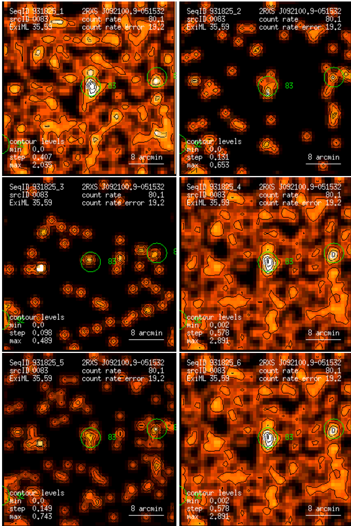
Figure 83: RASS 931825: detection 0083: band rate images, Gaussian filter: (1) PSPC channels 11 – 41, (2) 52 – 90, (3) 91 – 201, (4) 11 – 235, (5) 52 – 201, (6) 11 – 201. Broad band rates in counts/ks. Band rate contour levels in counts/ks/arcmin 2 .
