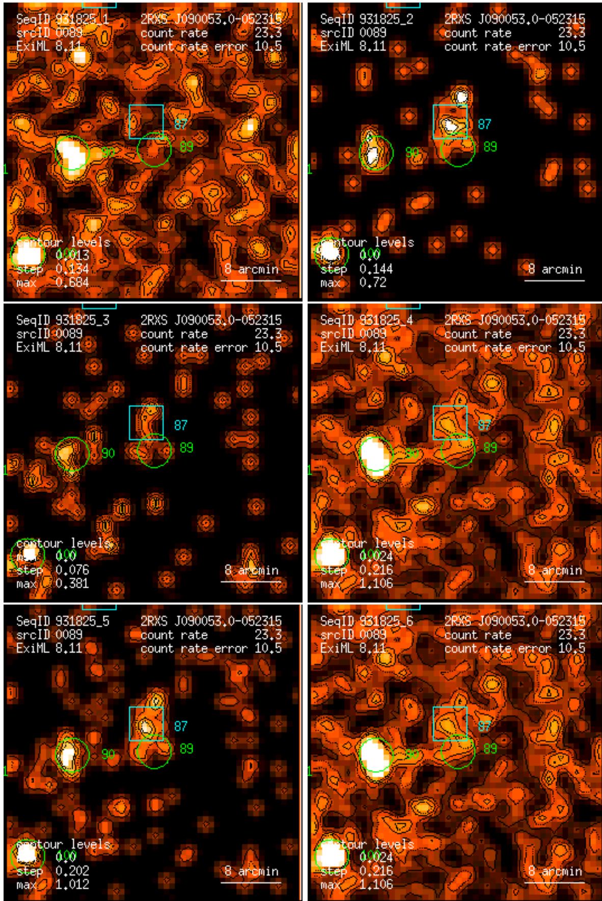
Figure 89: RASS 931825: detection 0089: band rate images, Gaussian filter: (1) PSPC channels 11 – 41, (2) 52 – 90, (3) 91 – 201, (4) 11 – 235, (5) 52 – 201, (6) 11 – 201. Broad band rates in counts/ks. Band rate contour levels in counts/ks/arcmin 2 .
