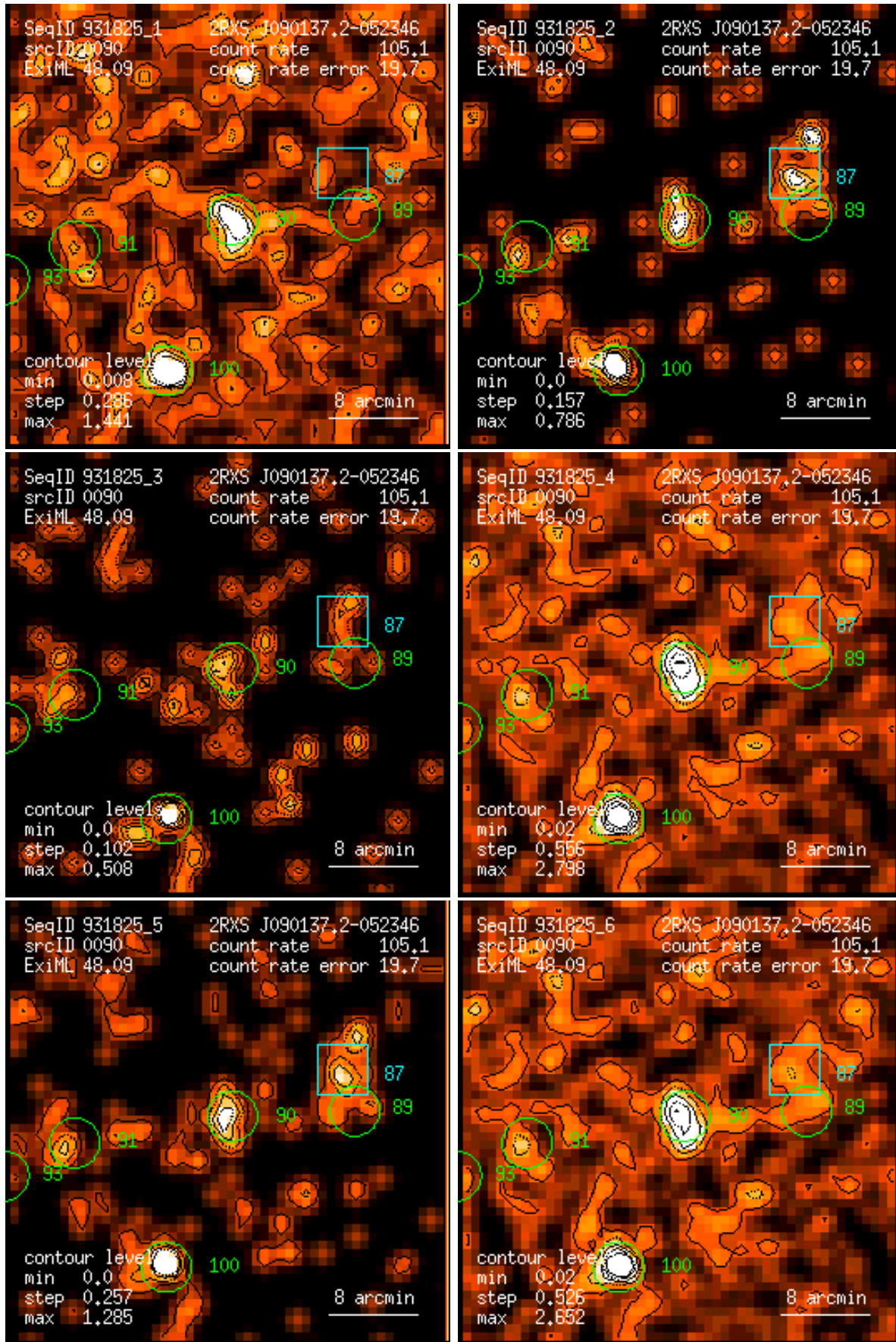
Figure 90: RASS 931825: detection 0090: band rate images, Gaussian filter: (1) PSPC channels 11 – 41, (2) 52 – 90, (3) 91 – 201, (4) 11 – 235, (5) 52 – 201, (6) 11 – 201. Broad band rates in counts/ks. Band rate contour levels in counts/ks/arcmin 2 .
