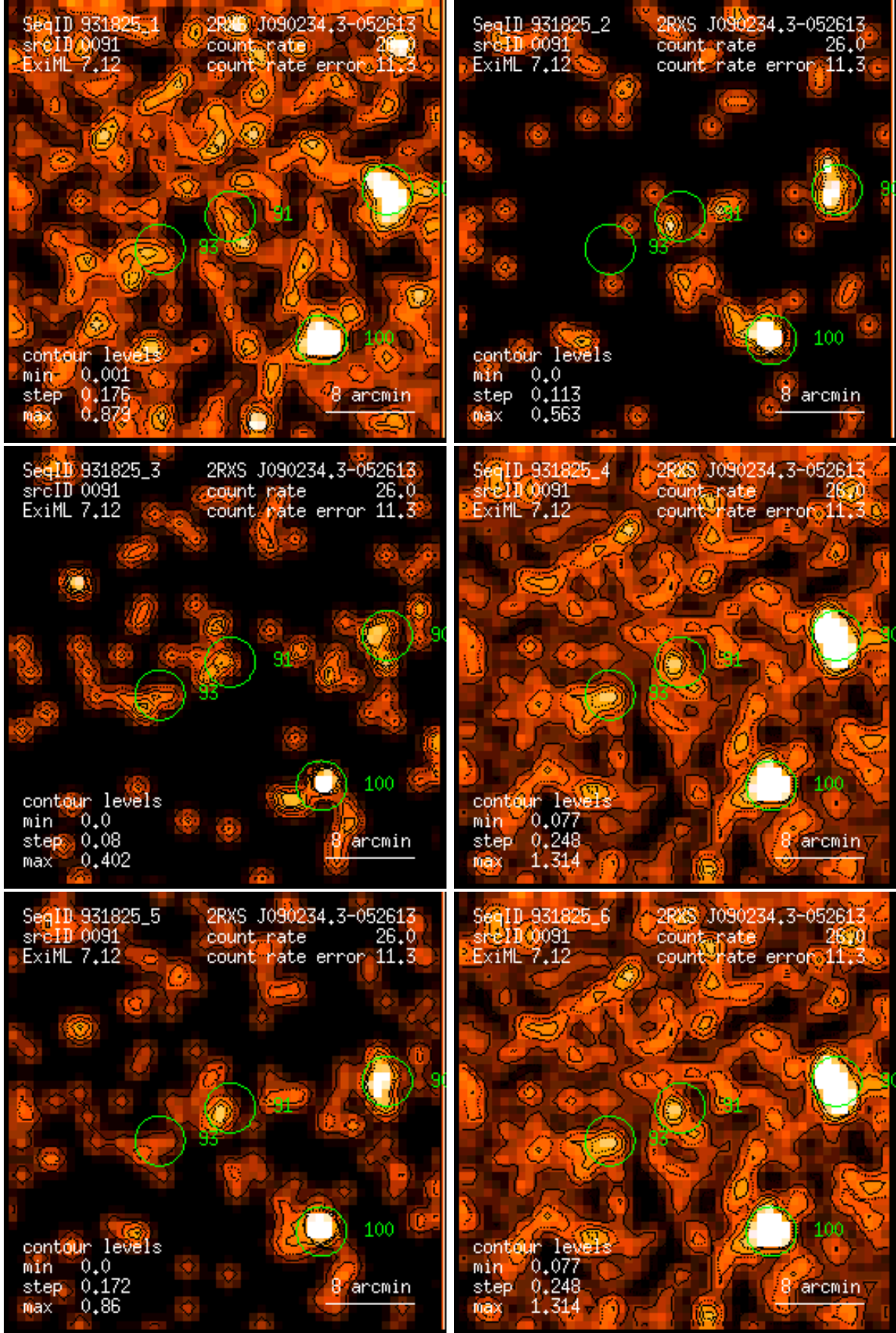
Figure 91: RASS 931825: detection 0091: band rate images, Gaussian filter: (1) PSPC channels 11 – 41, (2) 52 – 90, (3) 91 – 201, (4) 11 – 235, (5) 52 – 201, (6) 11 – 201. Broad band rates in counts/ks. Band rate contour levels in counts/ks/arcmin 2 .
