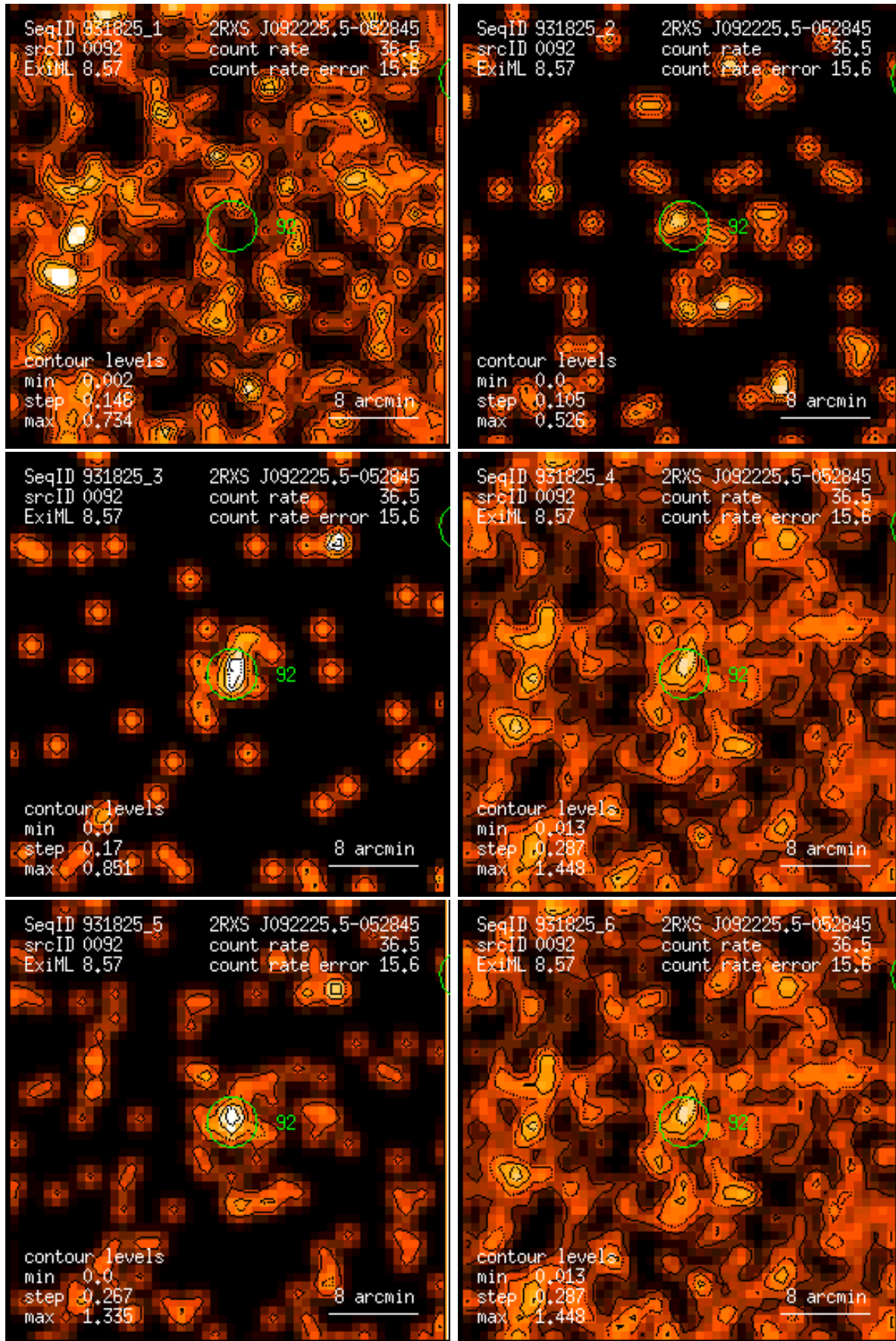
Figure 92: RASS 931825: detection 0092: band rate images, Gaussian filter: (1) PSPC channels 11 – 41, (2) 52 – 90, (3) 91 – 201, (4) 11 – 235, (5) 52 – 201, (6) 11 – 201. Broad band rates in counts/ks. Band rate contour levels in counts/ks/arcmin 2 .
