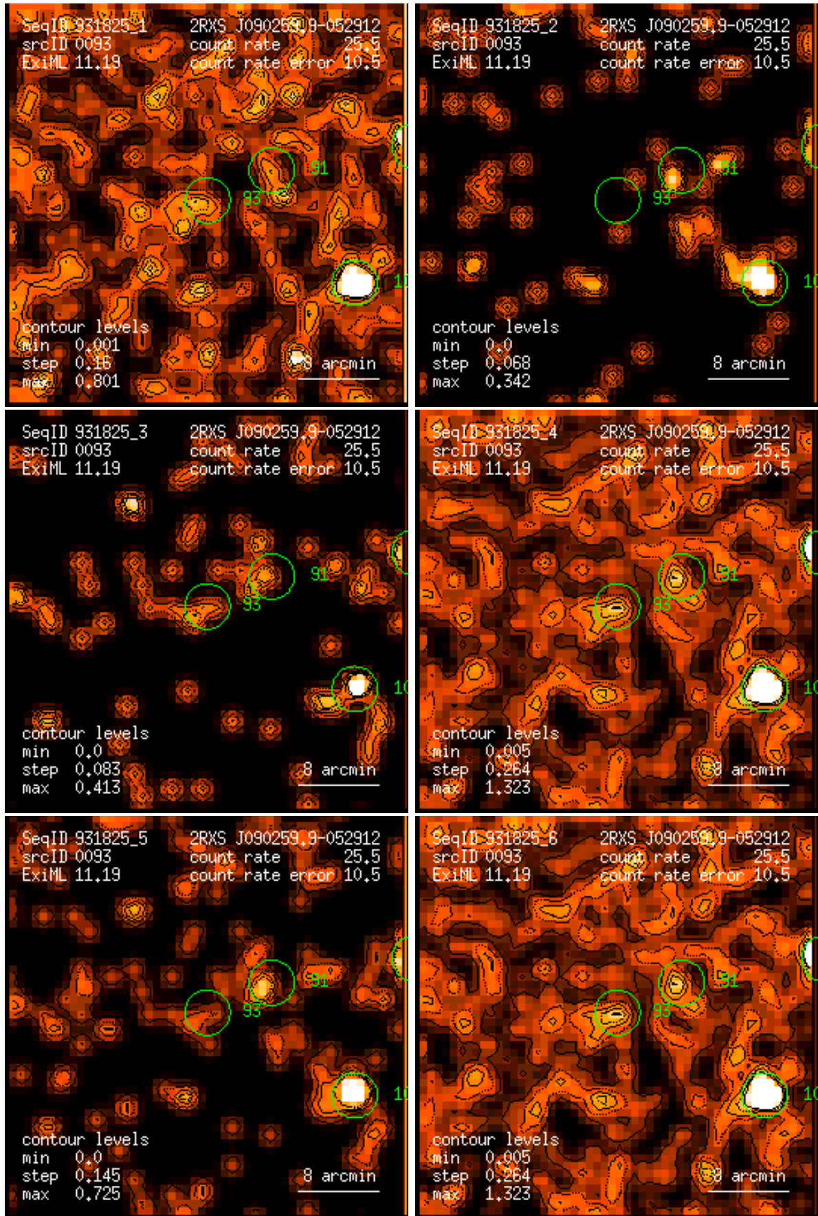
Figure 93: RASS 931825: detection 0093: band rate images, Gaussian filter: (1) PSPC channels 11 – 41, (2) 52 – 90, (3) 91 – 201, (4) 11 – 235, (5) 52 – 201, (6) 11 – 201. Broad band rates in counts/ks. Band rate contour levels in counts/ks/arcmin 2 .
